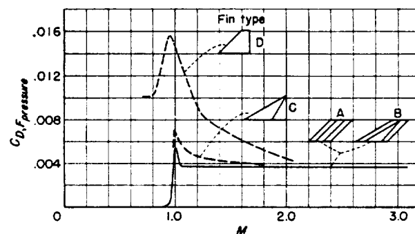
FIGURE 5.—Fin pressure drag coefficients (including base pressure) based on exposed fin area.
