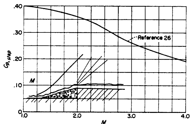
FIGURE 4.—Pressure coefficients on forward facing step for flow with turbulent boundary layer.
