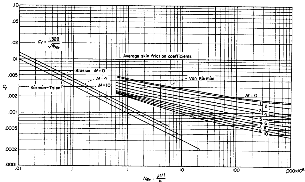
FIGURE 2.—Average skin-friction coefficients for flat plates based on wetted area.
