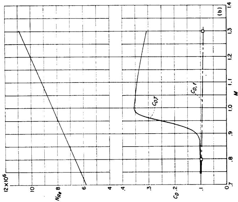
(b) N_{Re} and C_b curves.
