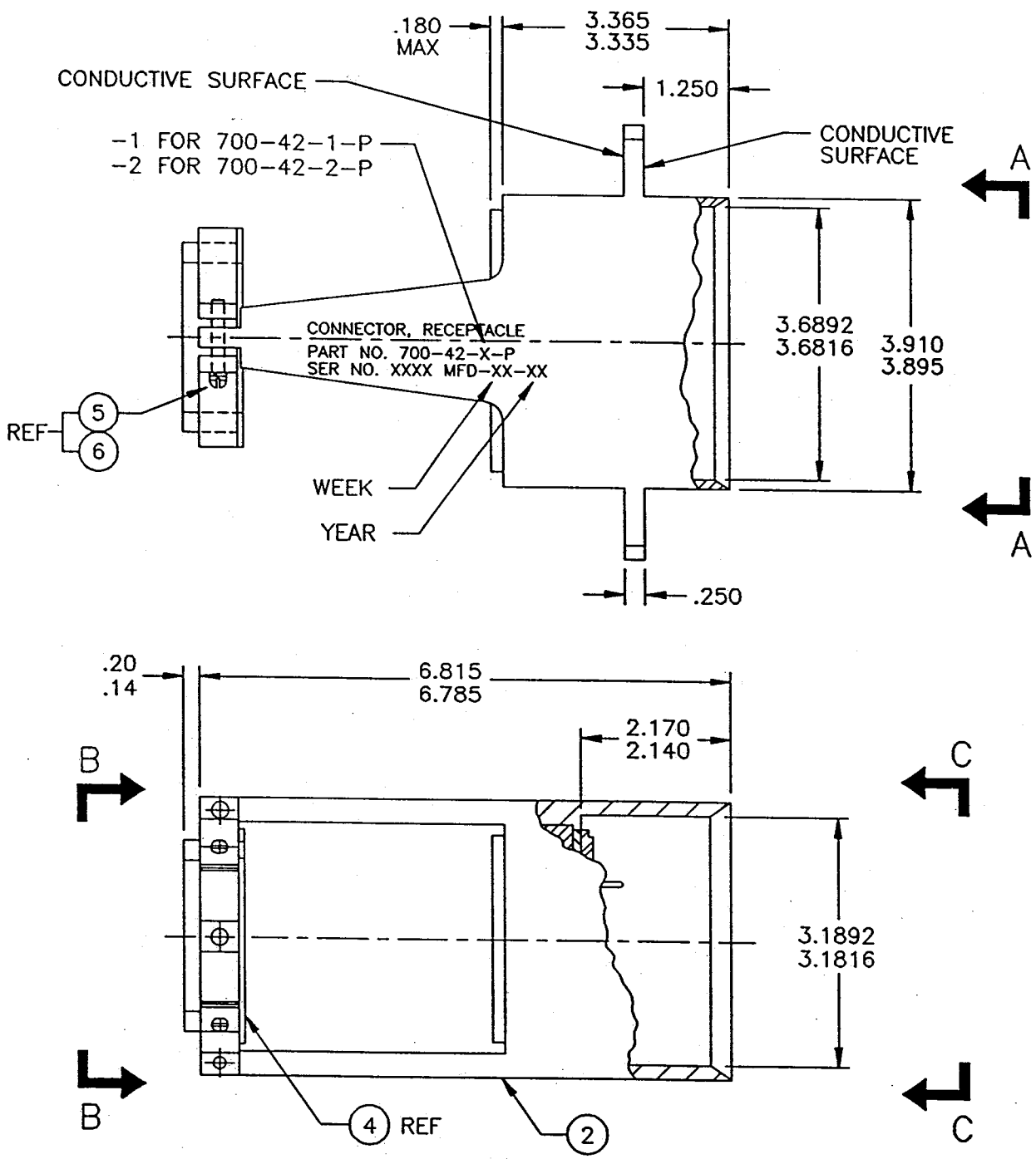
FIGURE 2B - CONNECTOR CONFIGURATION, CONNECTOR, RECEPTACLE, ELECTRICAL, RECTANGULAR (PAGE 1 OF 4)
