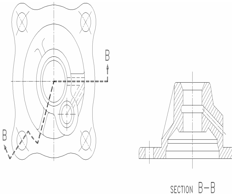
Figure 10: Offset Sections
