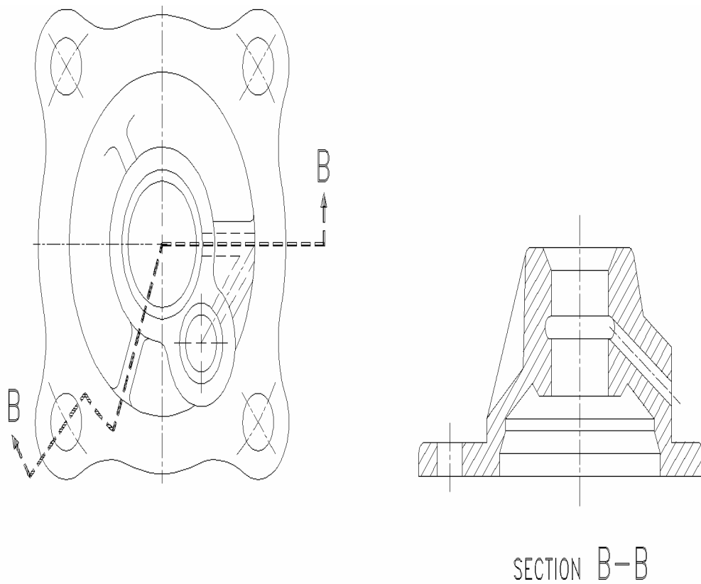
Figure 10: Offset Sections
