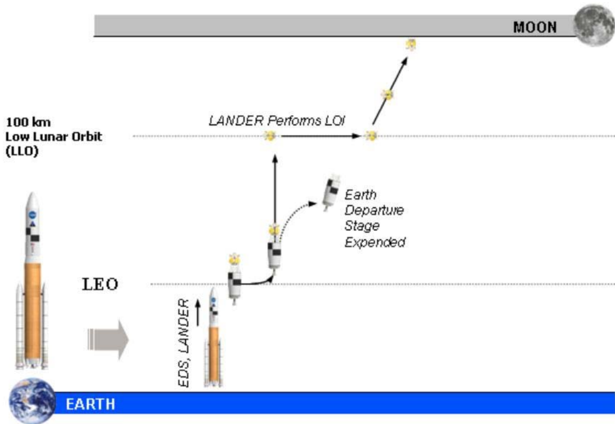
FIGURE 3.1.2-1 UNCREWED CARGO ALTAIR DRM
