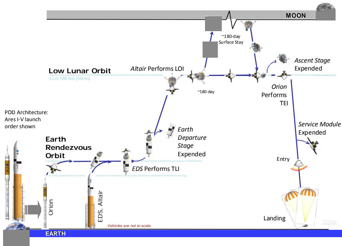
FIGURE 3.1.3-1 LUNAR OUTPOST – CREW DRM
