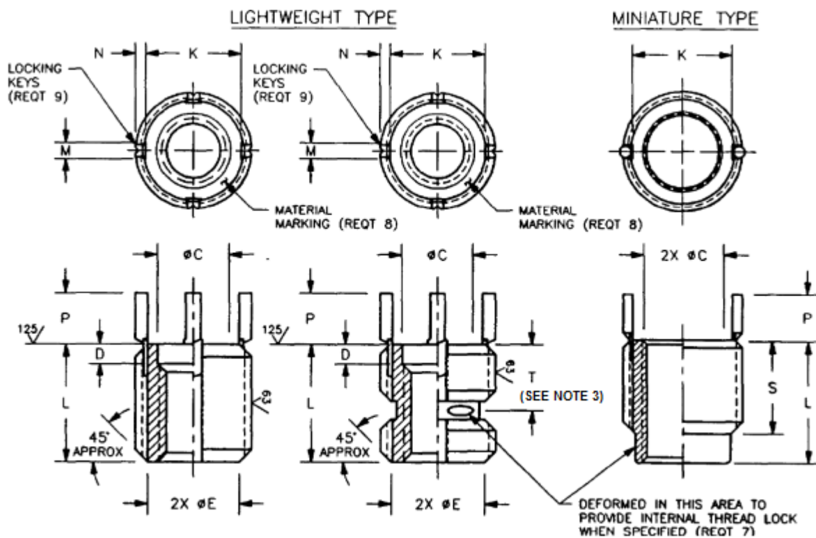
FIGURE 1. INSERT, COARSE INTERNAL THREADS.
