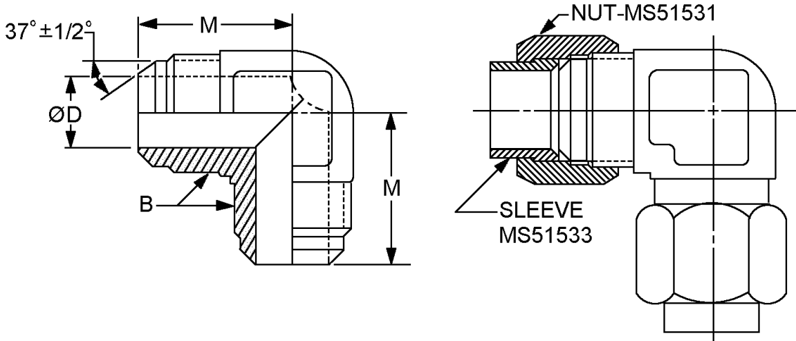
FIGURE 1. Elbow tube 90°.
