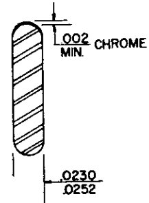
SECTION A-A ENLARGED
