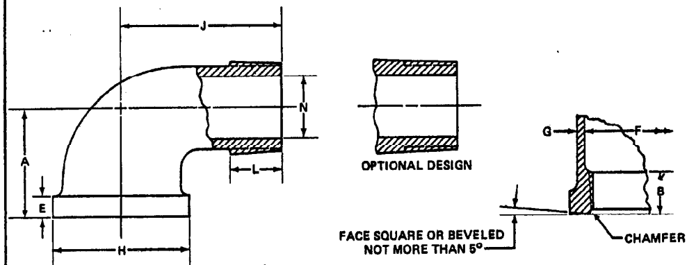
(B) Table I. Dimensions of Street Elbows - Class 150
