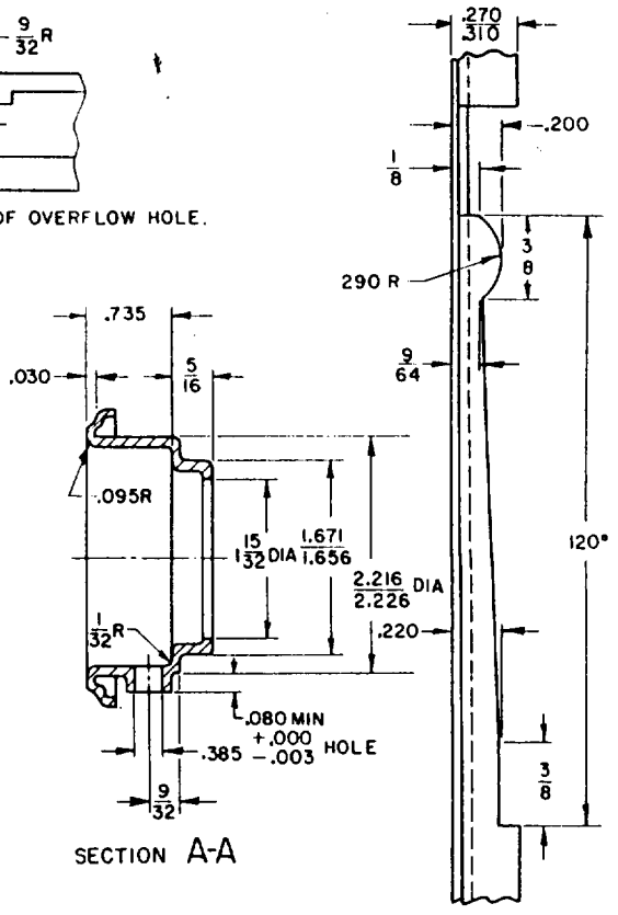
CAM DEVELOPMENT
