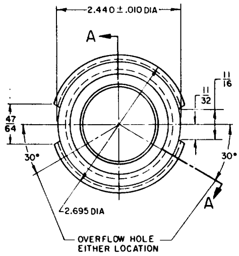
ENLARGED VIEW OF OVERFLOW HOLE. DESIGN OPTIONAL
