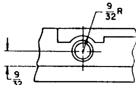
ENLARGED VIEW OF OVERFLOW HOLE. DESIGN OPTIONAL
