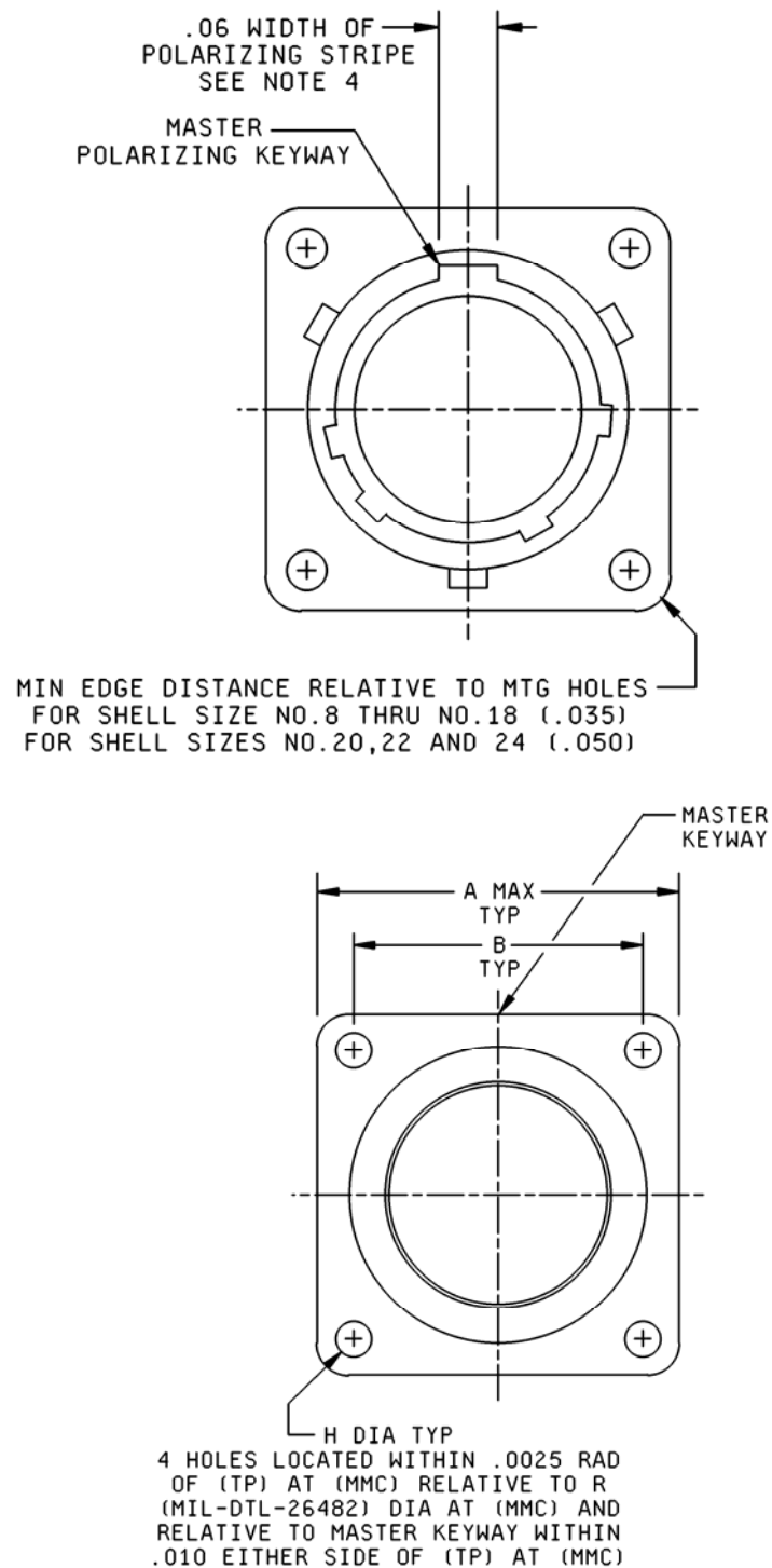
FIGURE 1. Receptacle, class N, dimensions and configurations - Continued.
