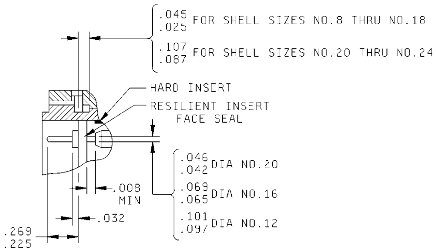
DETAIL T (COUPLING RING REMOVED FOR CLARITY)
