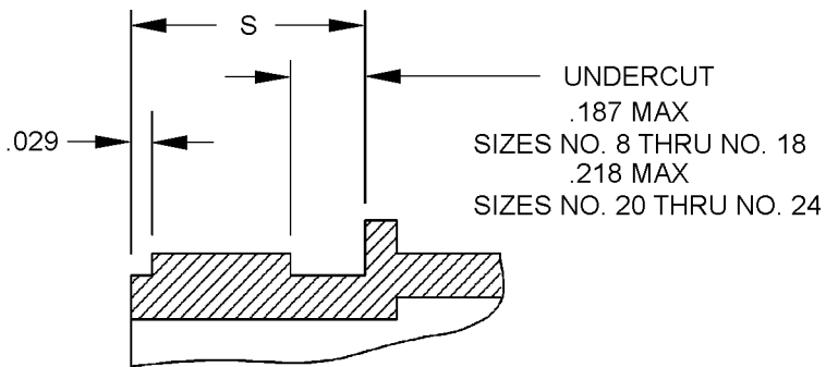
DETAIL T (COUPLING RING REMOVED FOR CLARITY)
