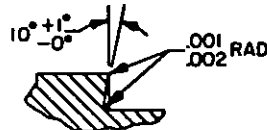
SECTIONAL VIEW OF DETAIL
