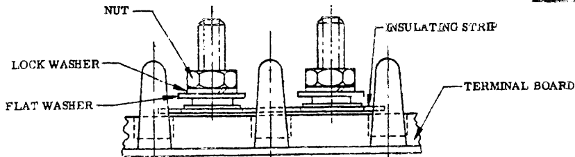
TYPICAL INSTALLATION
