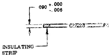
TYPICAL INSTALLATION
