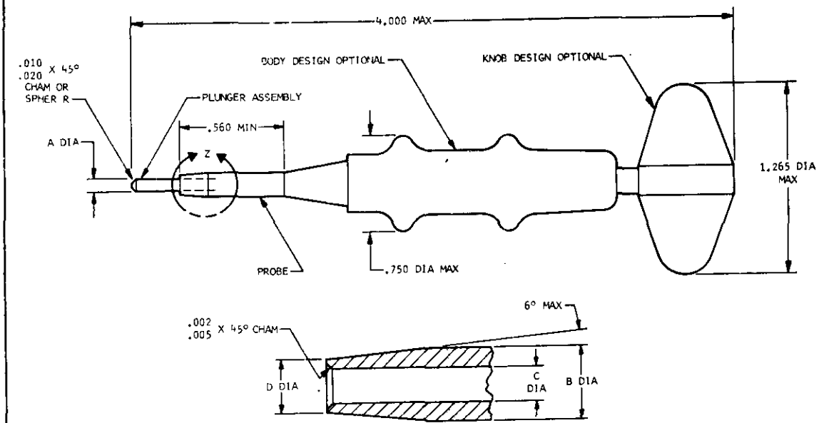
DETAIL Z (PROBE TIP)
