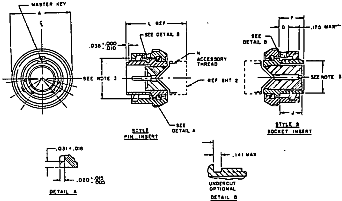
Classes E, F, J and P plugs
