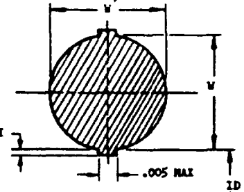
ENLARGED VIEW - SECTION A-A
