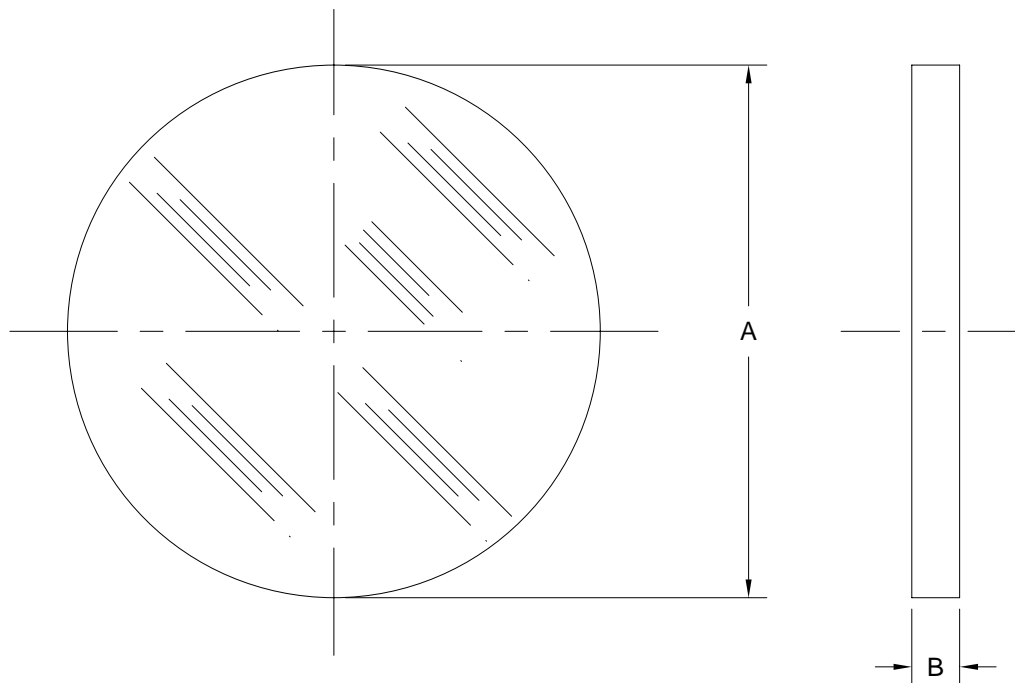
FIGURE 1. Cover Glass
