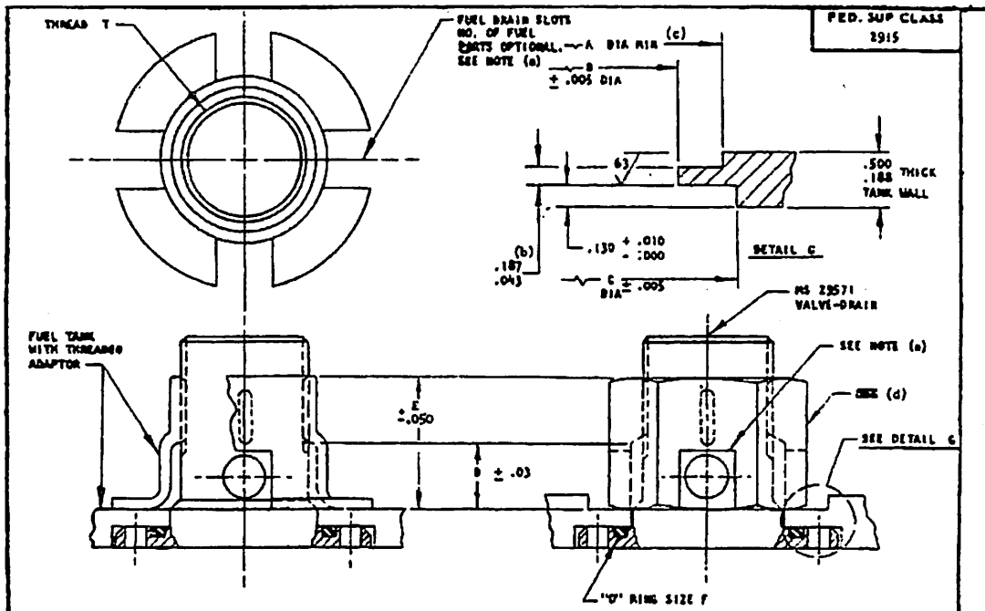
INSTALLATION PROVISIONS FOR MOUNTING DRAIN VALVE FROM OUTSIDE OF TANK
