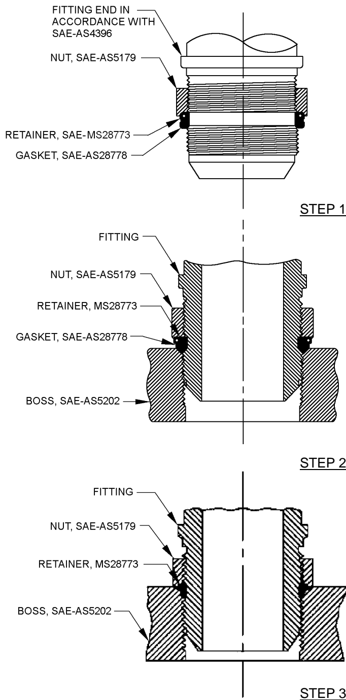
FIGURE 3. Positing type universal fitting installation.
