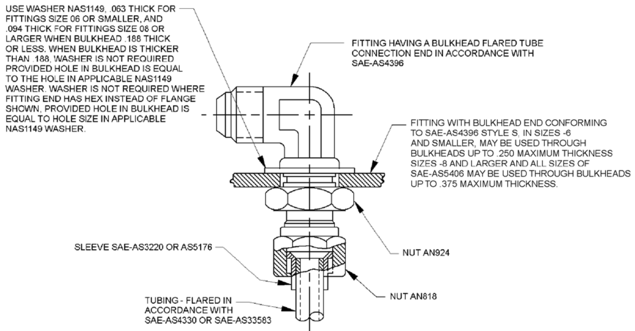
FIGURE 1. Bulkhead and flared tube installation.
