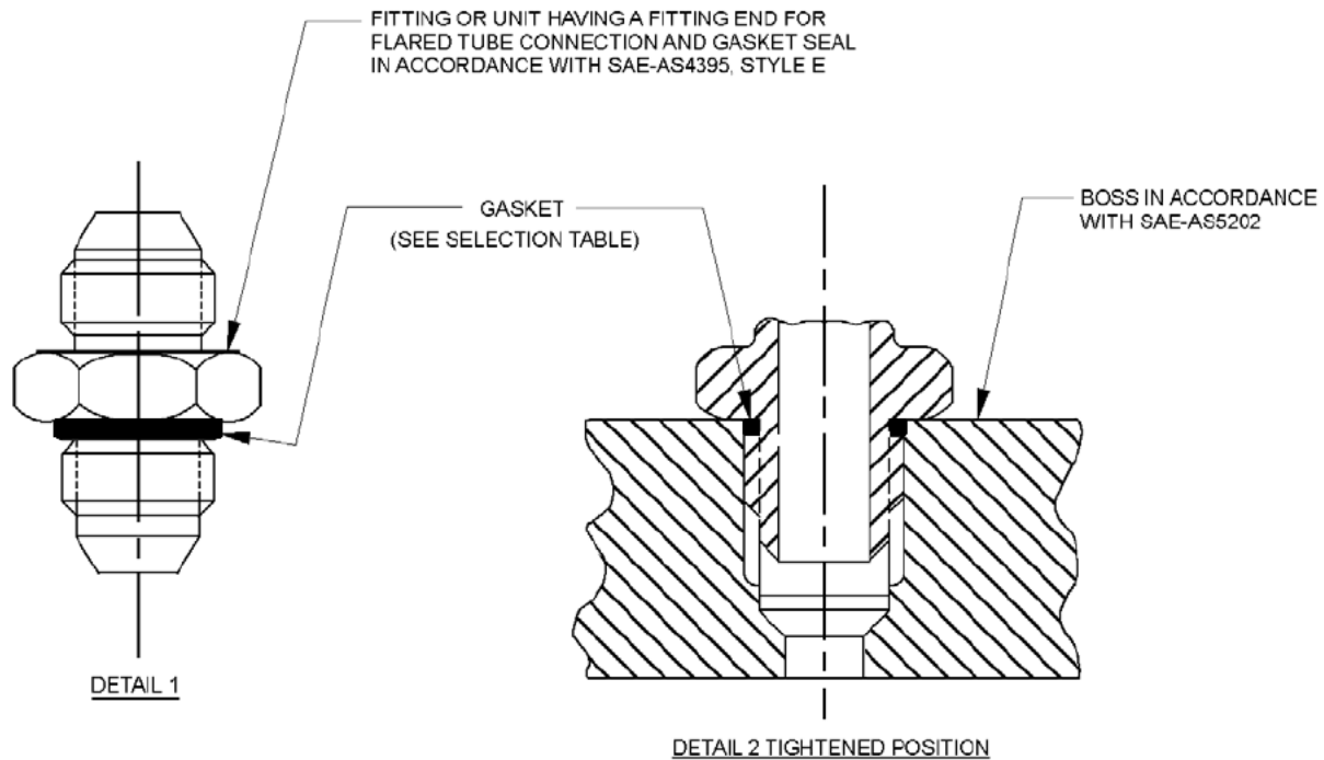
FIGURE 2. Non-positioning type fitting installation.
