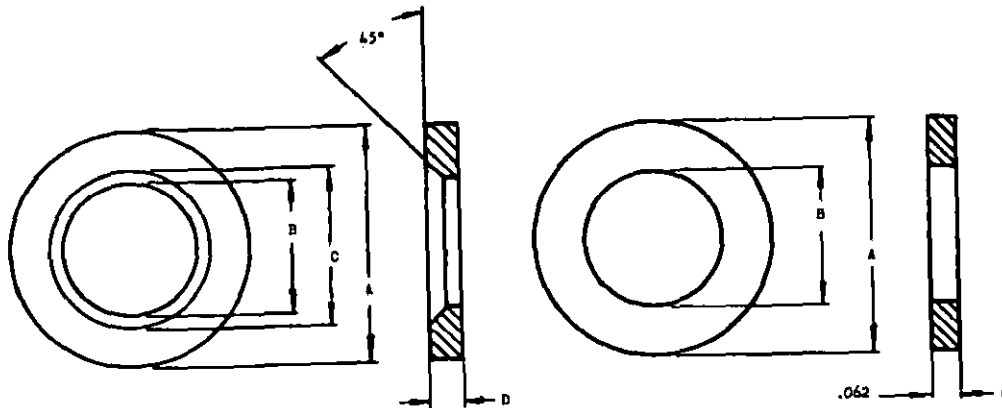
PLAIN WASHER (FOR USE UNDER NUT)
