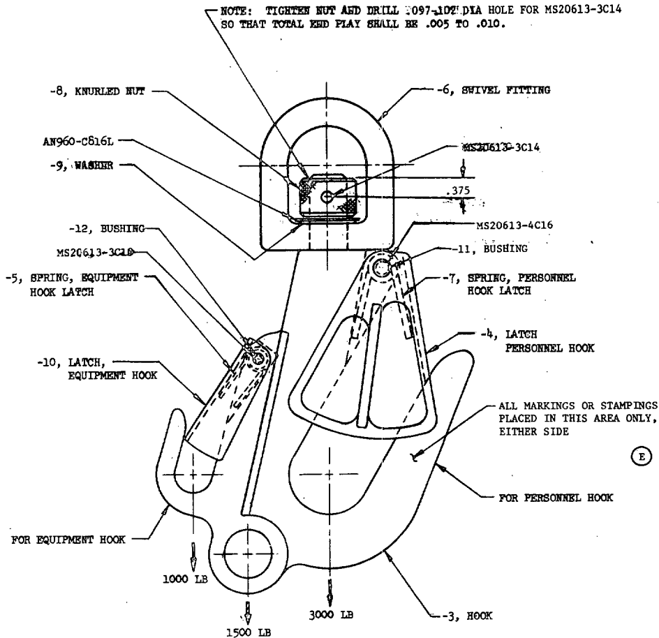
RESCUE HOOK ASSEMBLY
