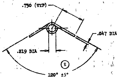
5. SPRING, PERSONNEL HOOK LATCH
