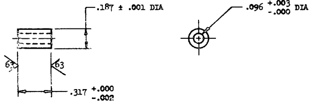
-12, BUSHING
