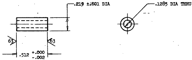
-11, BUSHING
