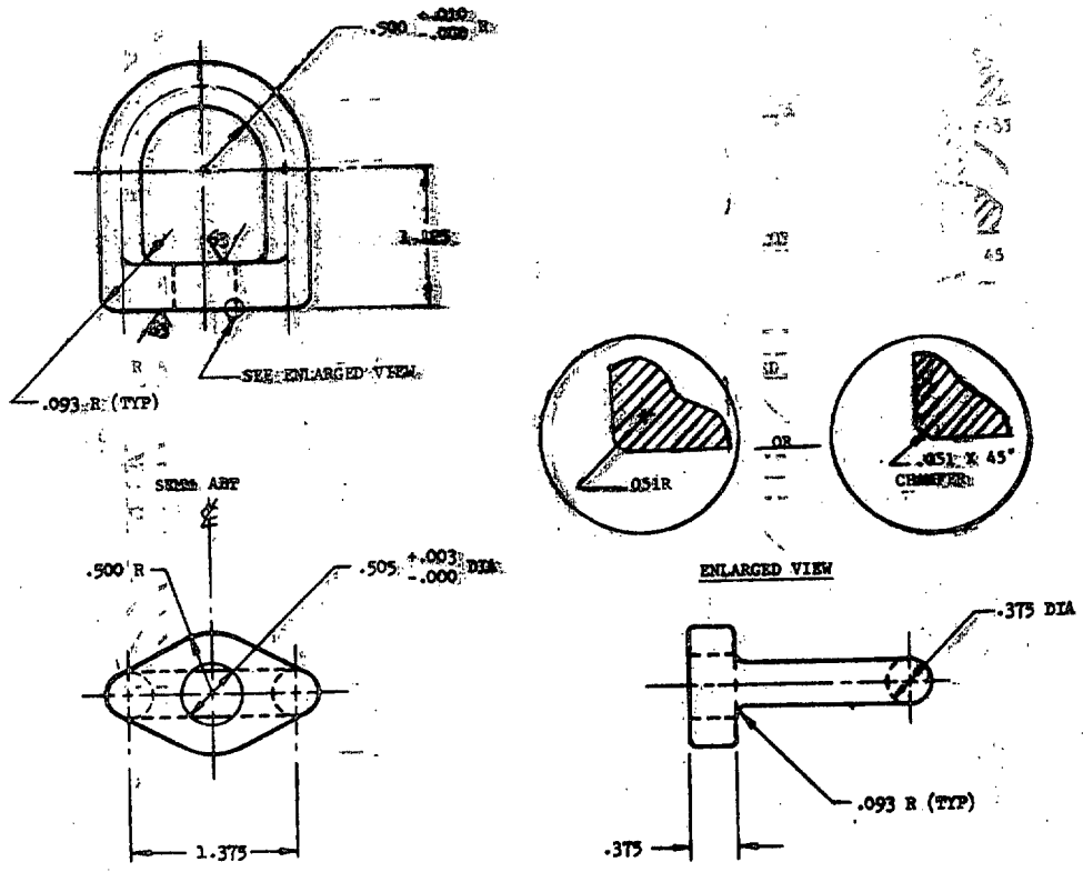
-6. SNIVEL FITTING
