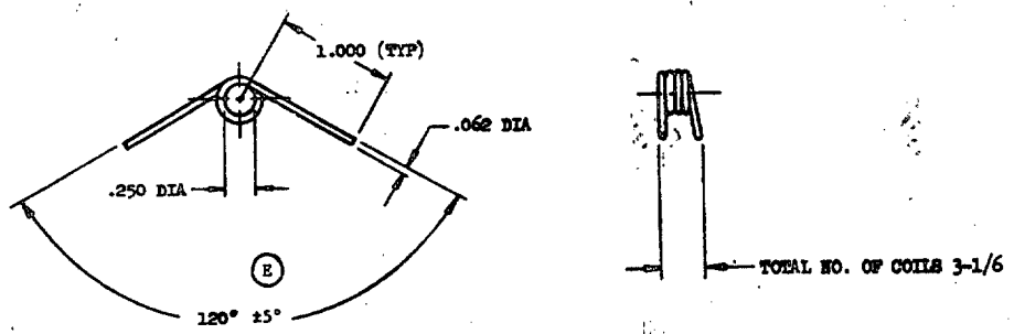
-7. SPRING, EMBOWED HOOK LATCH
