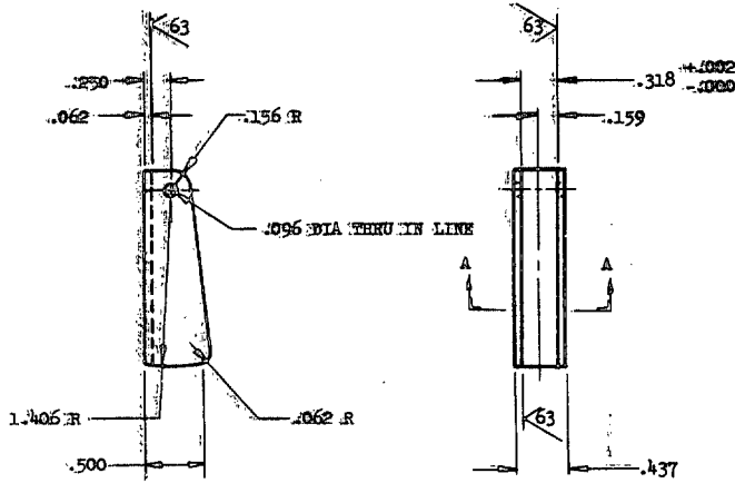
-10. LATCH EQUIPMENT HOOK
