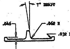
SECTION I-I
