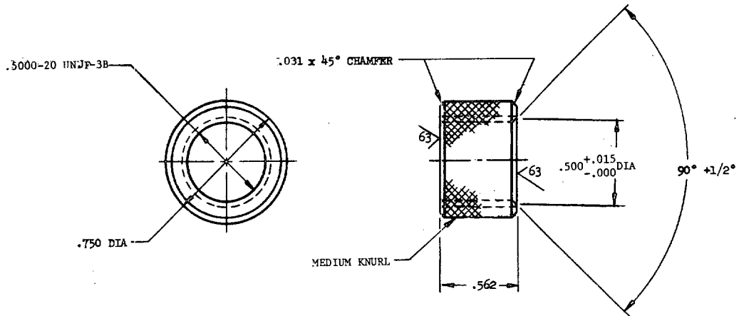
-8, KNURLED NUT
