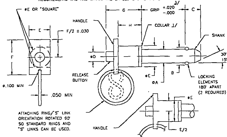
"T" HANDLE PIN, SINGLE ACTING
