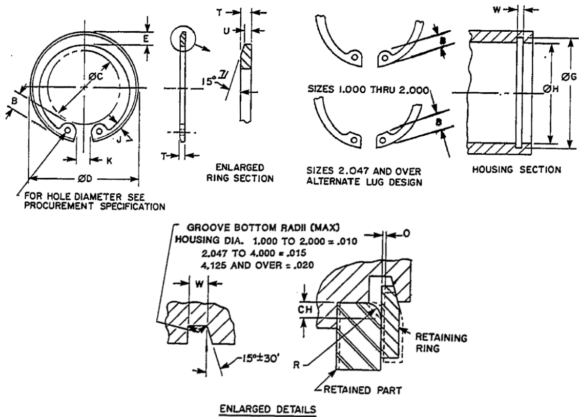
FIGURE 1. RING, RETAINING.
