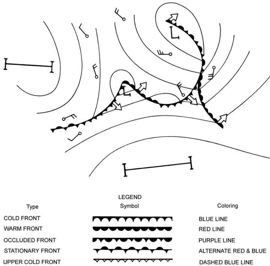
Figure 3425. Designation of fronts on weather maps.
