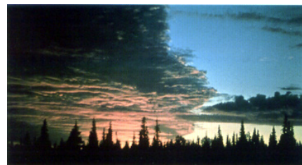
Figure 3615n. Altocumulus, one or more layers, mainly opaque, not expanding, or Altocumulus with Altostratus or Nimbostratus.
