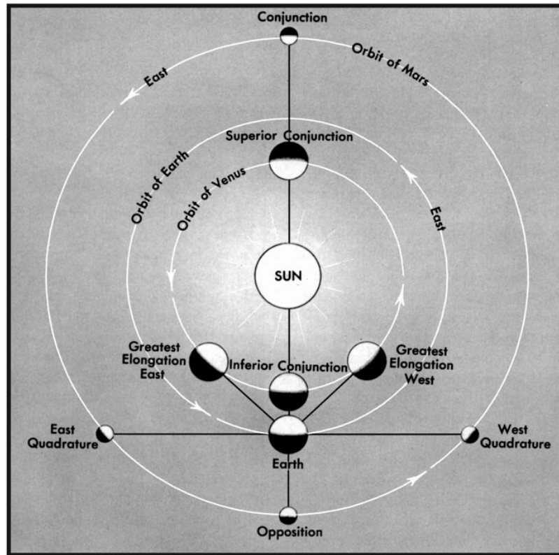
Figure 1510. Planetary configurations.
