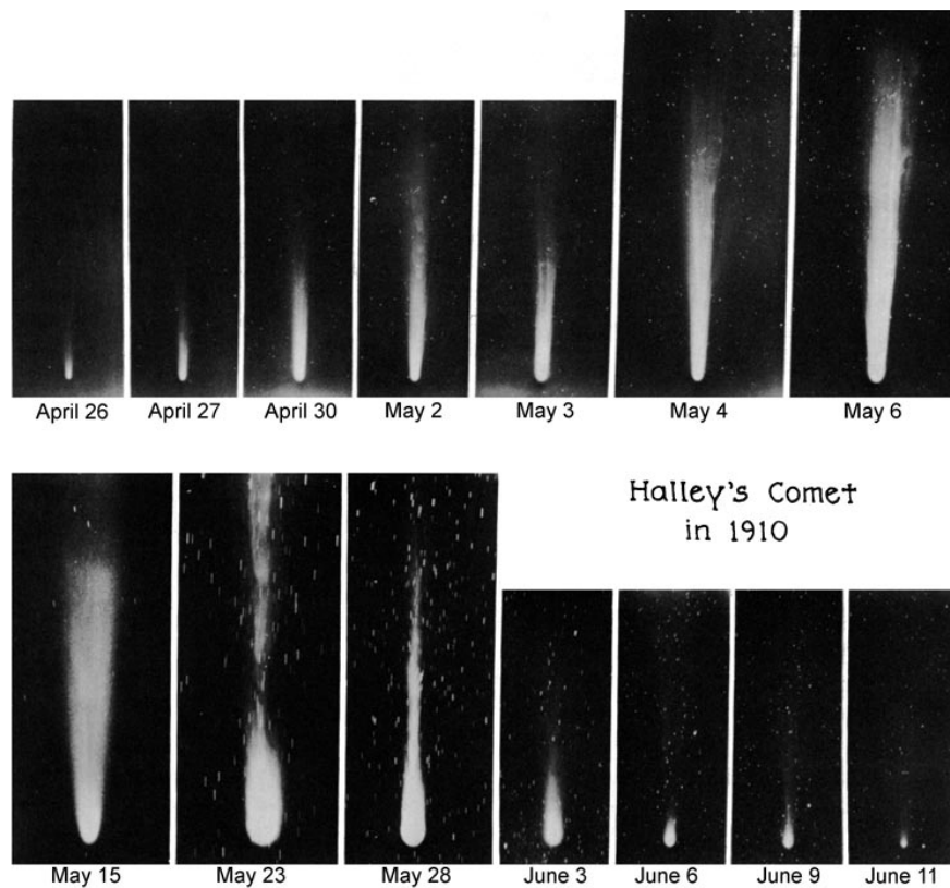
Figure 1513. Halley's Comet; fourteen views, made between April 26 and June 11, 1910.
