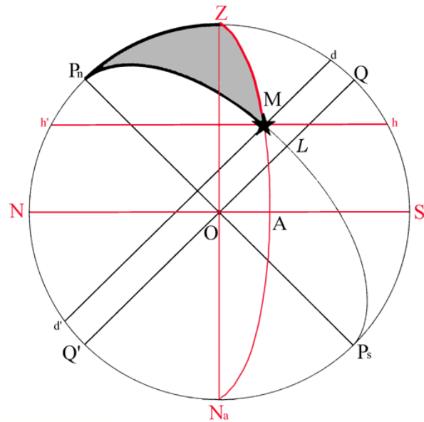
Figure 1529a. The navigational triangle.
