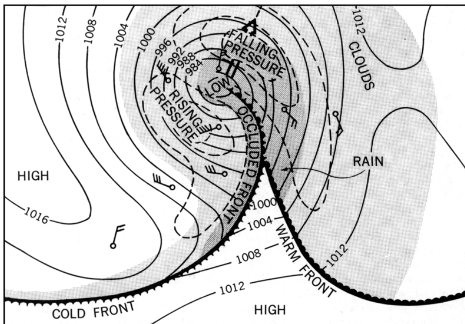
Figure 3410d. An occluded front (top view).
