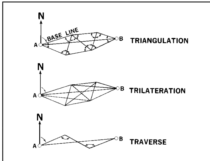
Figure 206. Triangulation, trilateration, and traverse.
