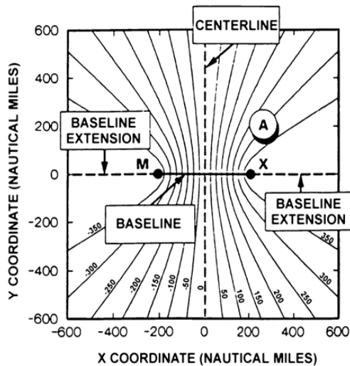
Figure 1204. Depiction of Loran LOP's.
