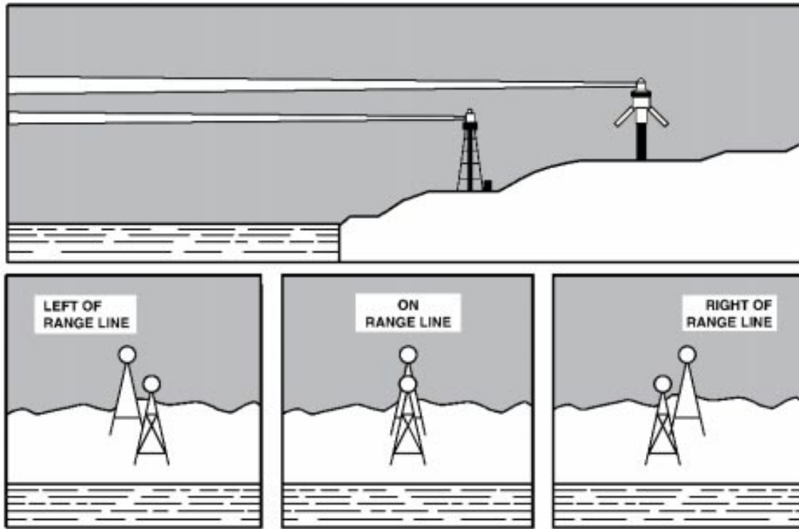
Figure 502. Range lights.
