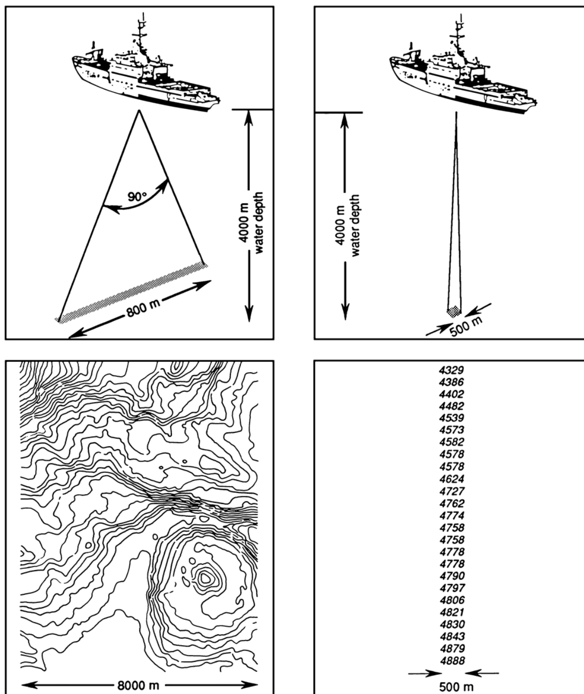
Figure 2905. Swath versus single-transducer surveys.
