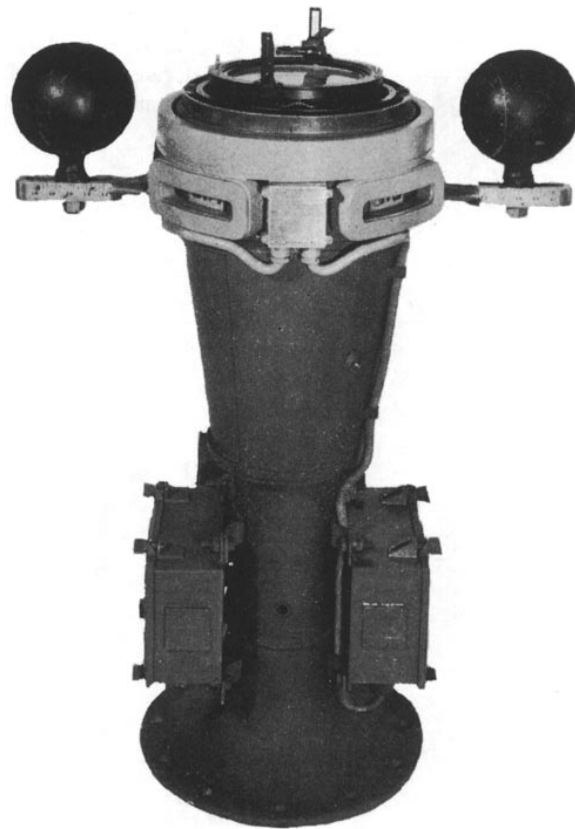
Figure 616. Type K degaussing compensation installation.
