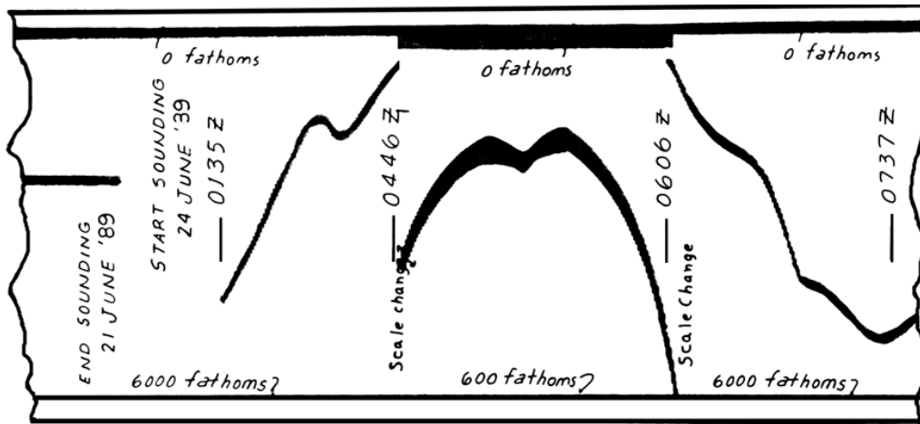
Figure 2916a. Annotated echo sounding record.
