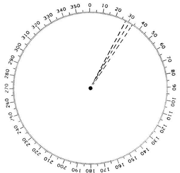
Figure 1308c. Ramark appears as broken radial line.
