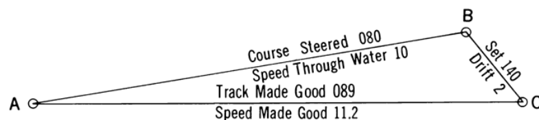
Figure 707. Determining an estimated position.
