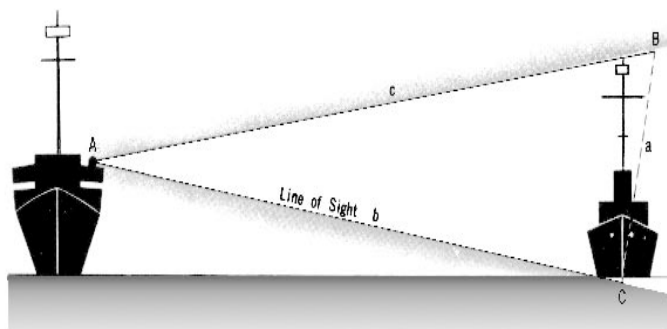
Figure 811c. Principle of stadimeter operation.
