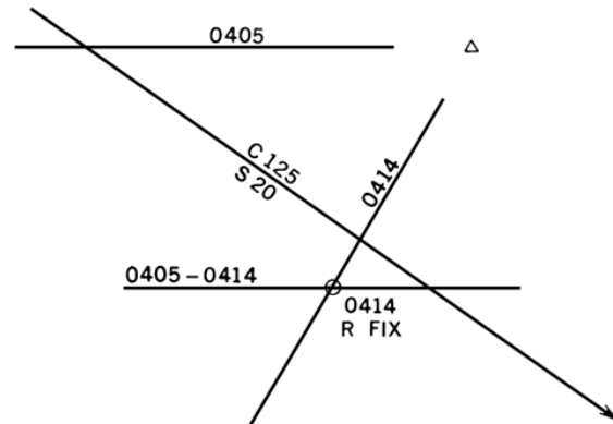
Figure 812e. A running fix by two bearings on the same object.
