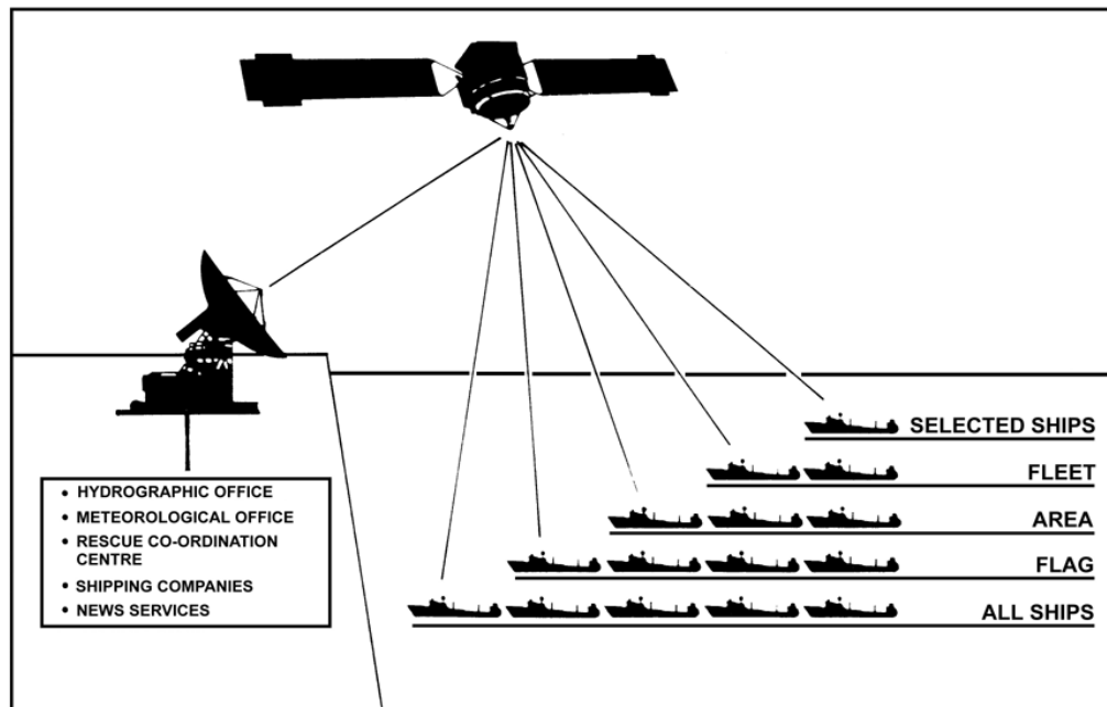
Figure 2805. SafetyNET EGC concept.
