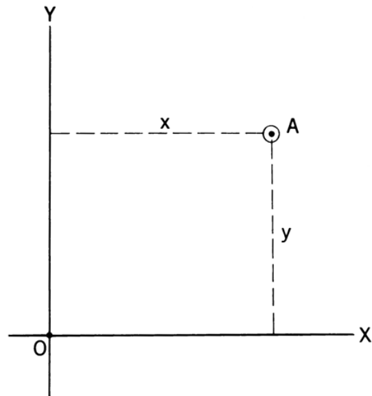
Figure 2105. Rectangular coordinates.
