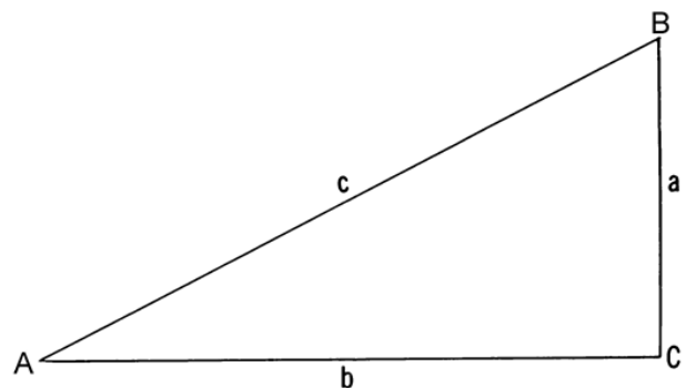
Figure 2108b. A right triangle.
