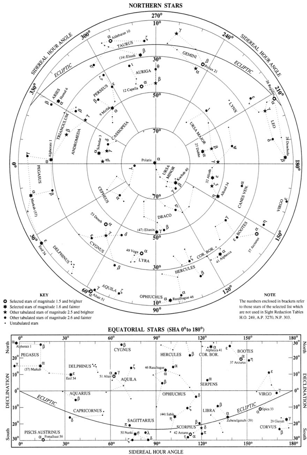
Figure 1532a. Star chart from Nautical Almanac.
