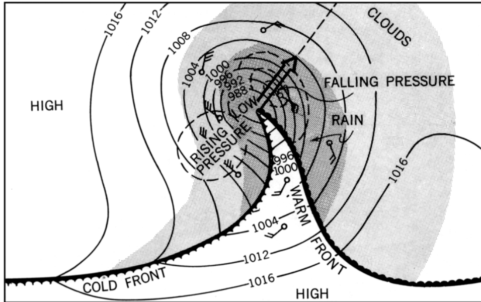
Figure 3410c. A frontal wave nearing occlusion (top view).
