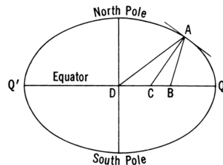
Figure 1523. Three kinds of latitude at point A.
