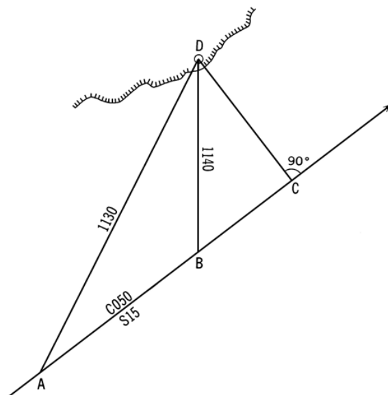
Figure 821. Triangles involved in a Table 18 running fix.
