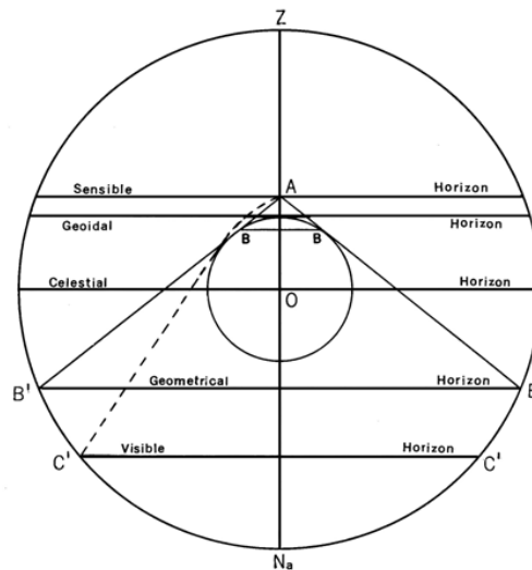
Figure 1526. The horizons used in navigation.
