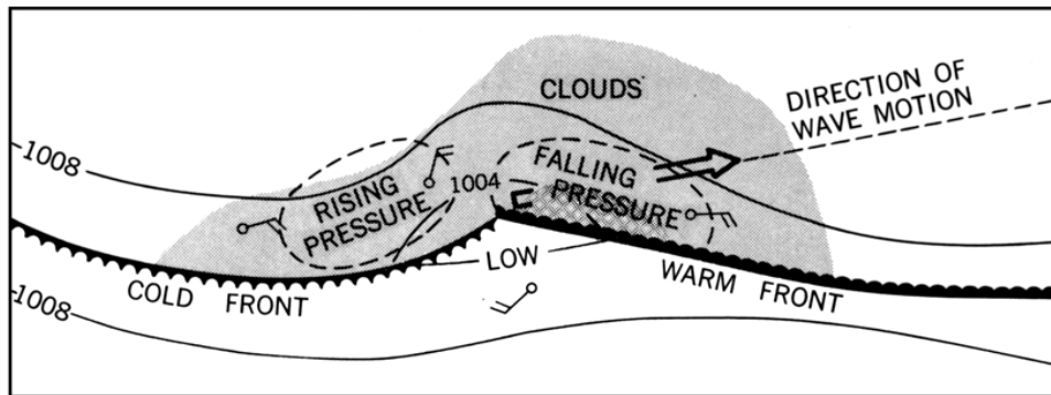
Figure 3410a. First stage in the development of a frontal wave (top view).
