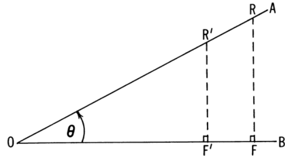
Figure 2108a. Similar right triangles.
