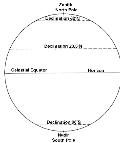
Figure 1516b. The parallel sphere.
