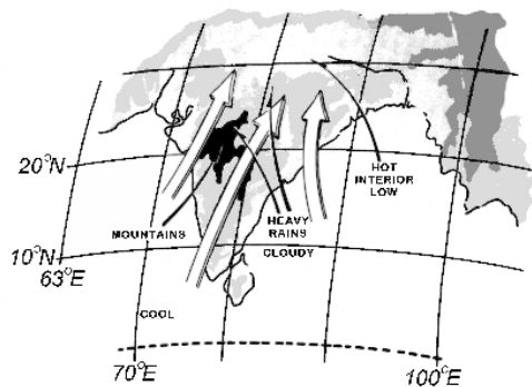
Figure 3408a. The summer monsoon.
