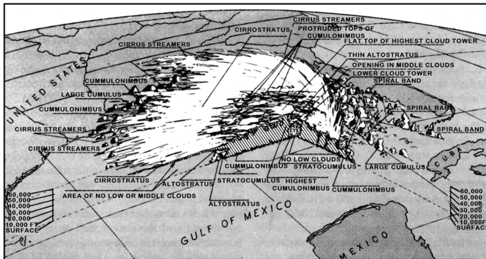
Figure 3508. Typical hurricane cloud formations.
