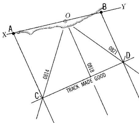
Figure 820b. Determining the track made good.
