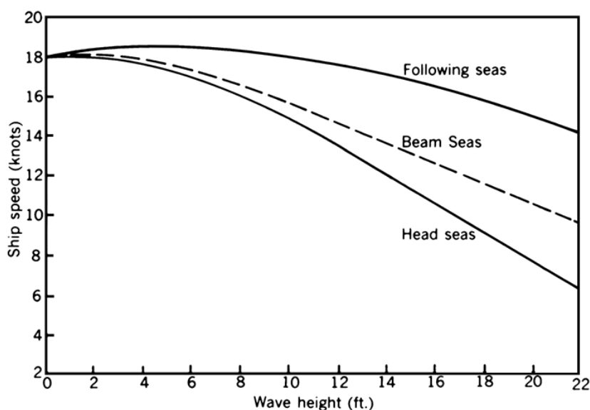
Figure 3703. Performance curves for head, beam, and following seas.
