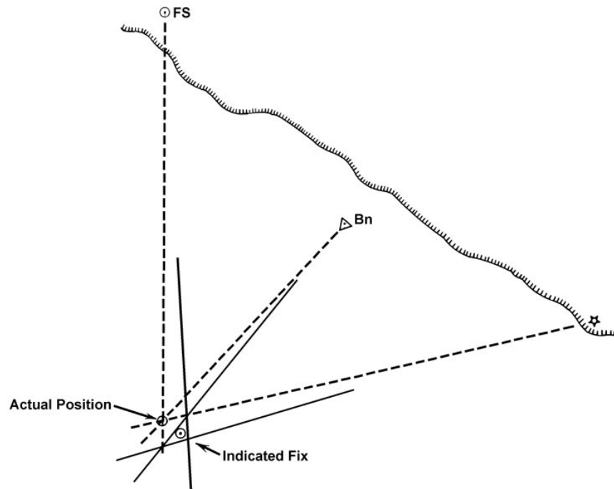
Figure 824. Adjusting a fix for constant error.
