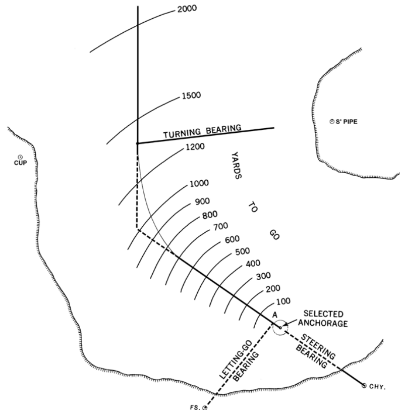
Figure 817. Anchoring.
