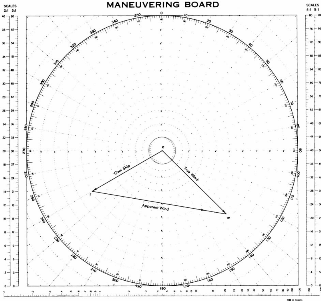
Figure 3609. Finding true wind by Maneuvering Board.
