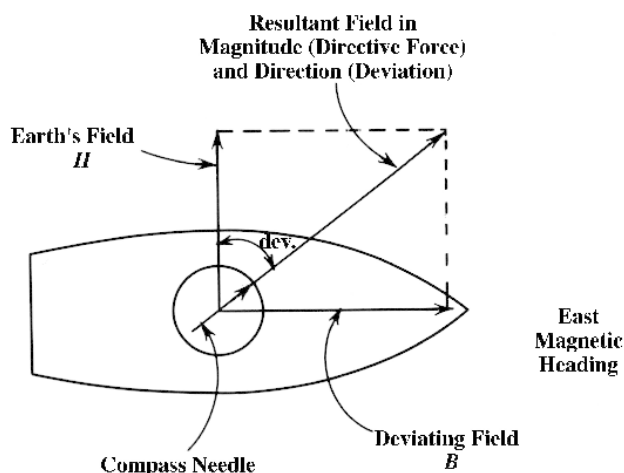
Figure 604c. General force diagram.
