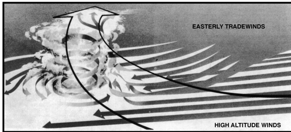
Figure 3504. Pumping action of high-altitude winds.
