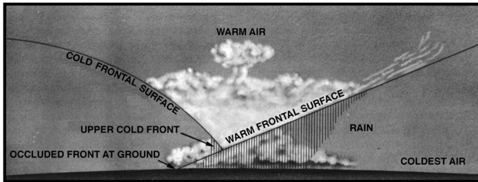
Figure 3410e. An occluded front (cross section).
