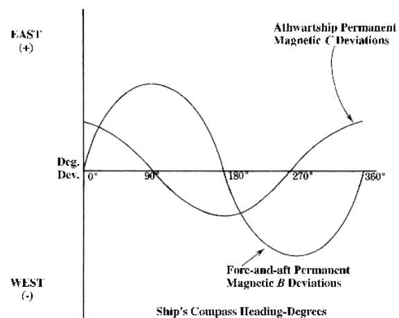
Figure 604b. Permanent magnetic deviation effects.
