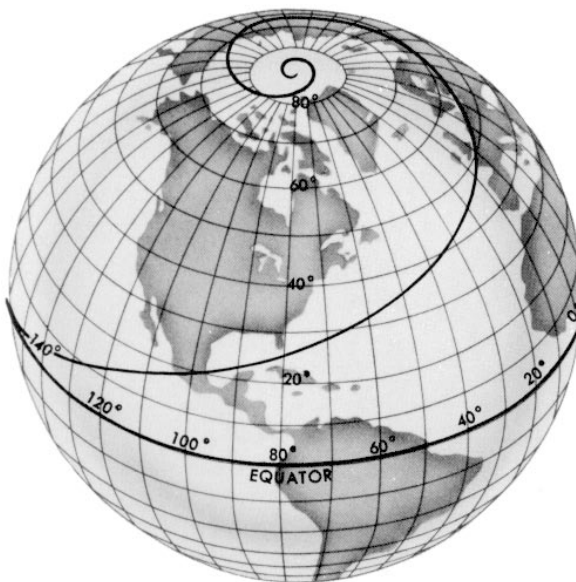
Figure 106. A loxodrome.
