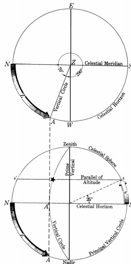
Figure 1528b. Measurement of horizon system of coordinates.
