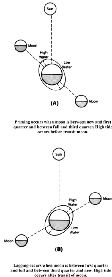
Figure 908c. Priming and lagging the tides.
