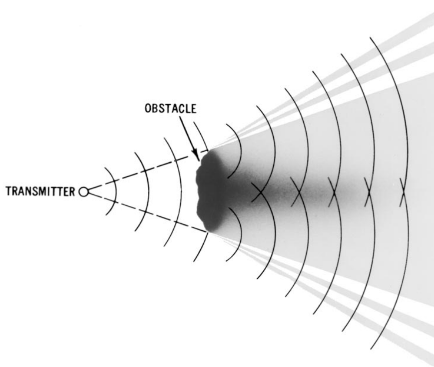
Figure 1008. Diffraction.
