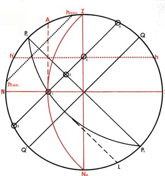
Figure 1528d. A diagram on the plane of the celestial meridian for lat. 45^\circ N .
