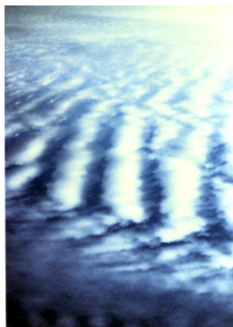
Figure 3615j. Altocumulus, one or more bands or layers, expanding, thickening.
