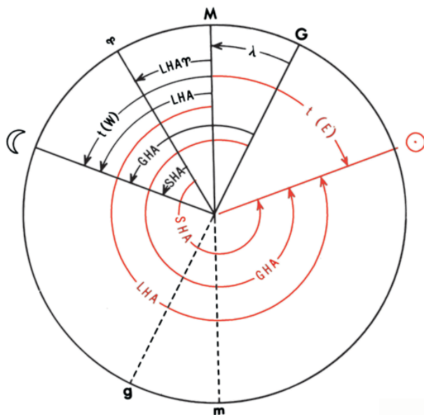
Figure 1525b. Time diagram.
