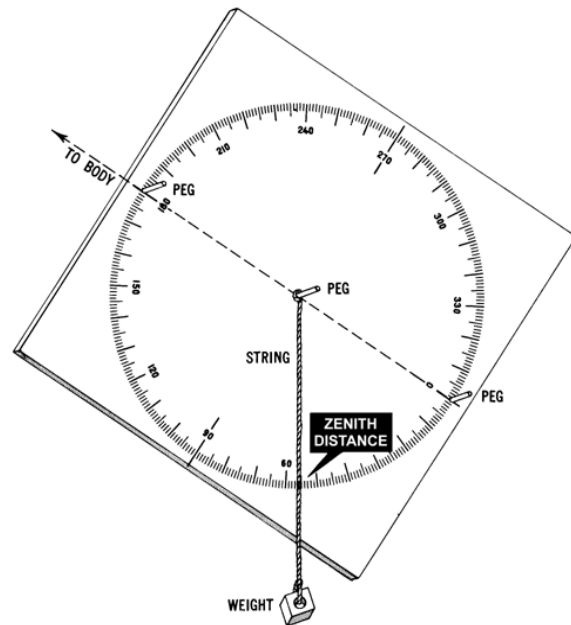
Figure 2608b. Improvised astrolabe; direct sighting method.
