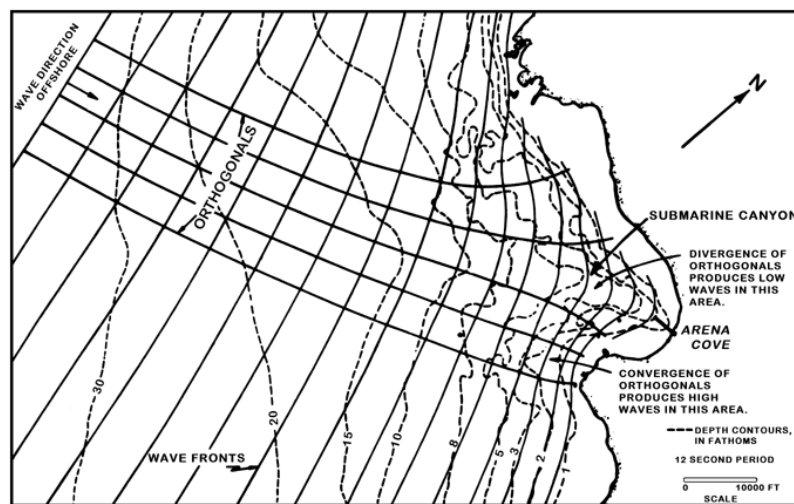
Figure 3215. The effect of bottom topography in causing wave convergence and wave divergence.
