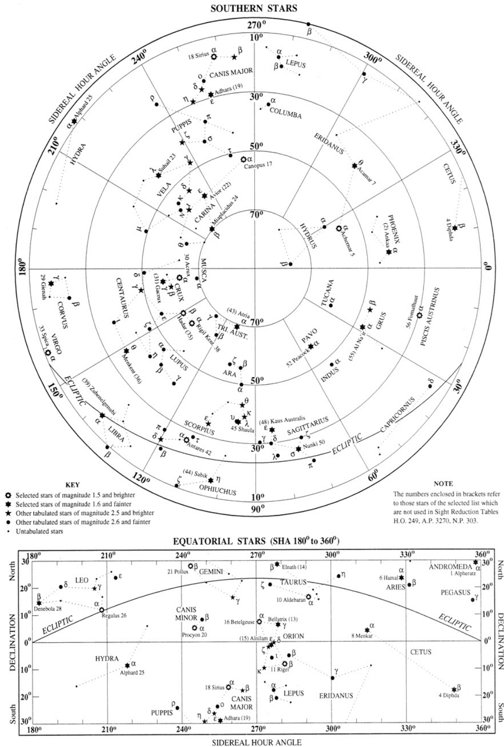
Figure 1532b. Star chart from Nautical Almanac.
