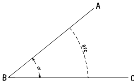
Figure 2101. An angle.
