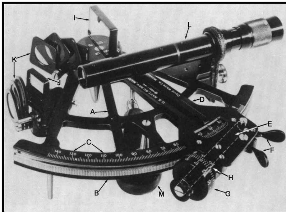
Figure 1602. U.S. Navy Mark 2 micrometer drum sextant.
