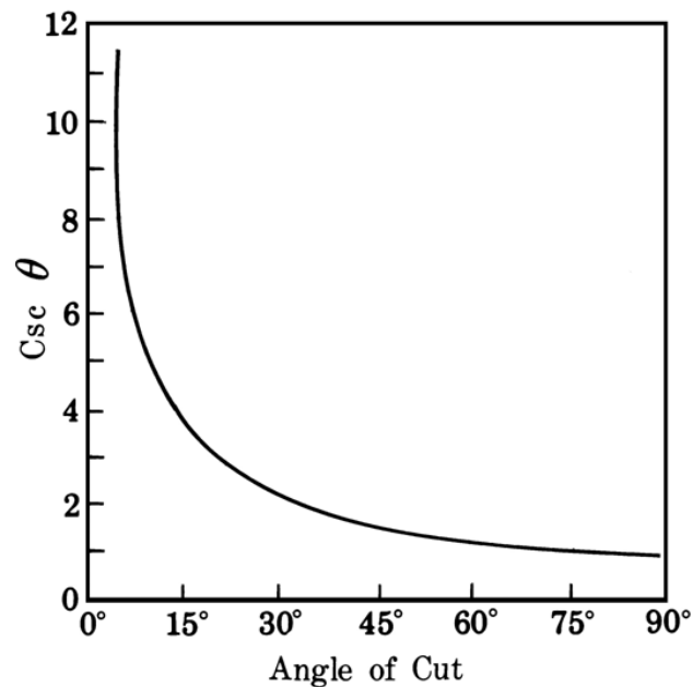
Figure 823c. Error of two-bearing plot.
