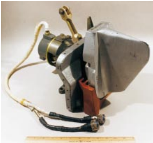
Figure 2-31: A jet vane for a liquid rocket.
