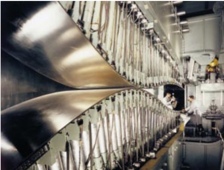
Figure 15-8: Exposed adjustable nozzle section of wind tunnel.
