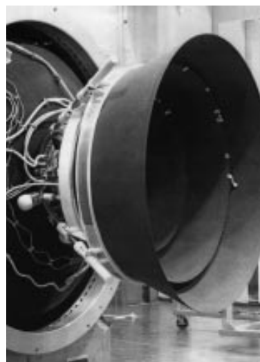
Figure 3-23: A modern extendable rocket nozzle skirt showing the actuators that increase its length after staging.
