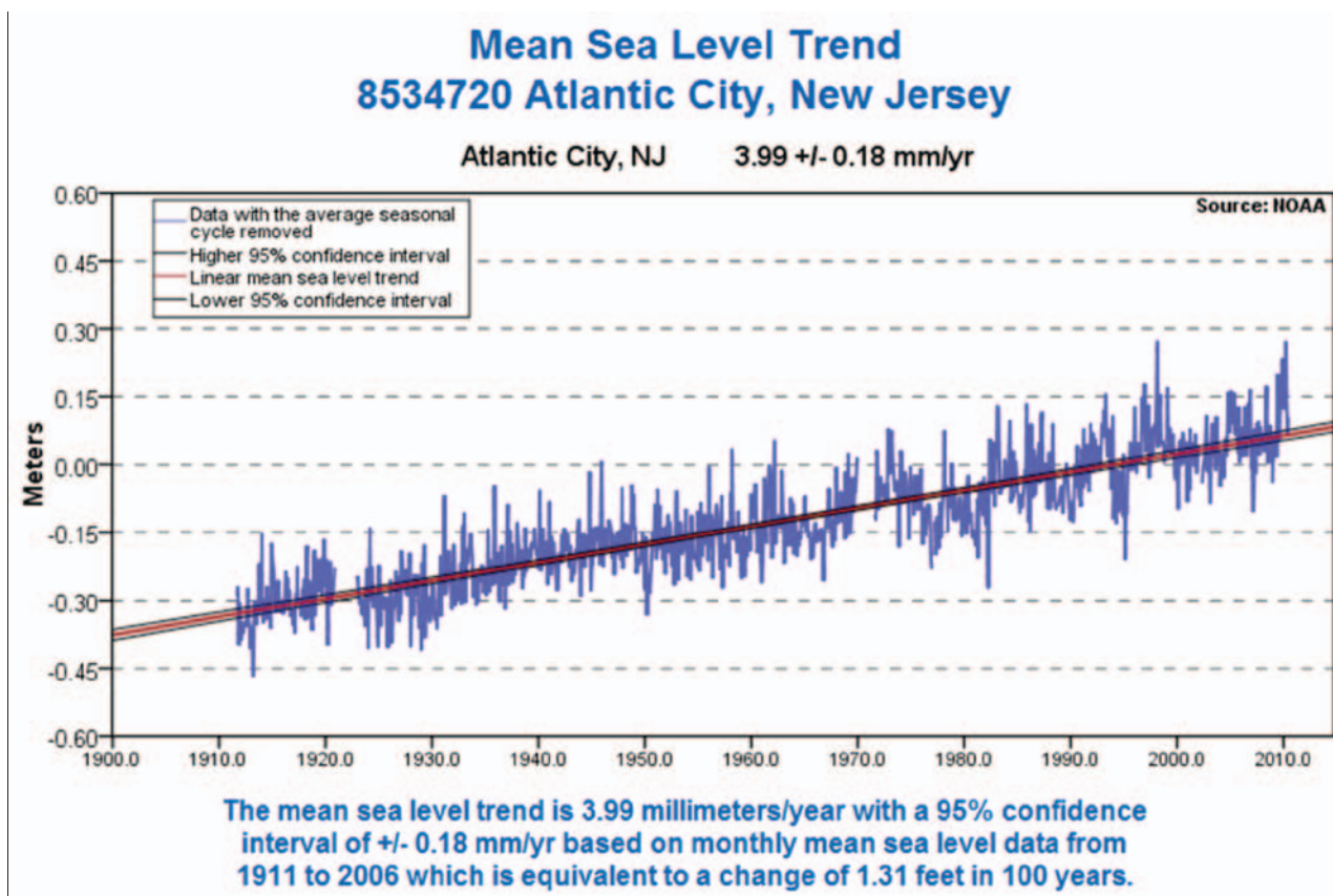
Figure 3-14. Mean sea level rise data for a station in Atlantic City, NJ
