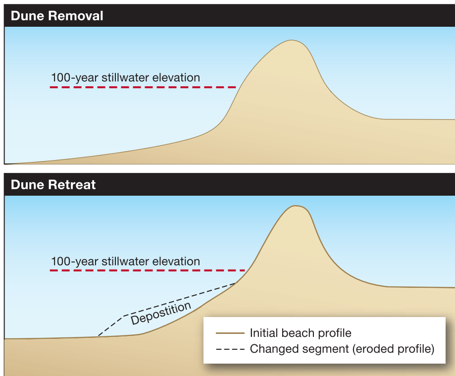
Figure 3-58. Current FEMA treatment of dune removal and dune retreat
