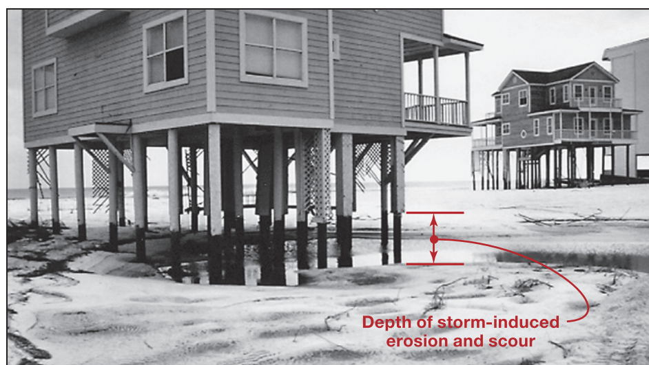
Figure 3-21. Pile-supported house in the area of channeled flow shown in Figure 3-20. The building foundation and elevation successfully prevented high-velocity flow, erosion, and scour from destroying this building
