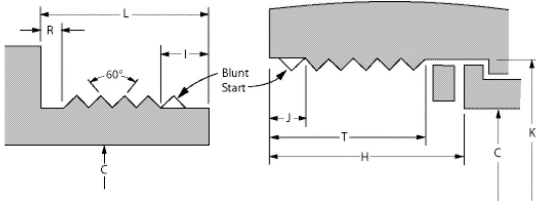
Figure 1—Thread and gasket recess configuration.
