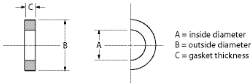
Figure 2—Gasket configuration.
