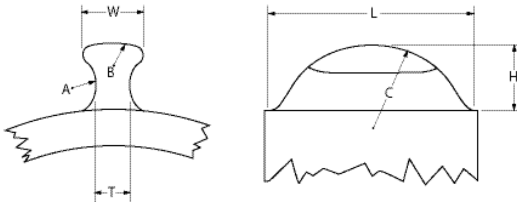
Figure 3—Rocker lug configuration.
