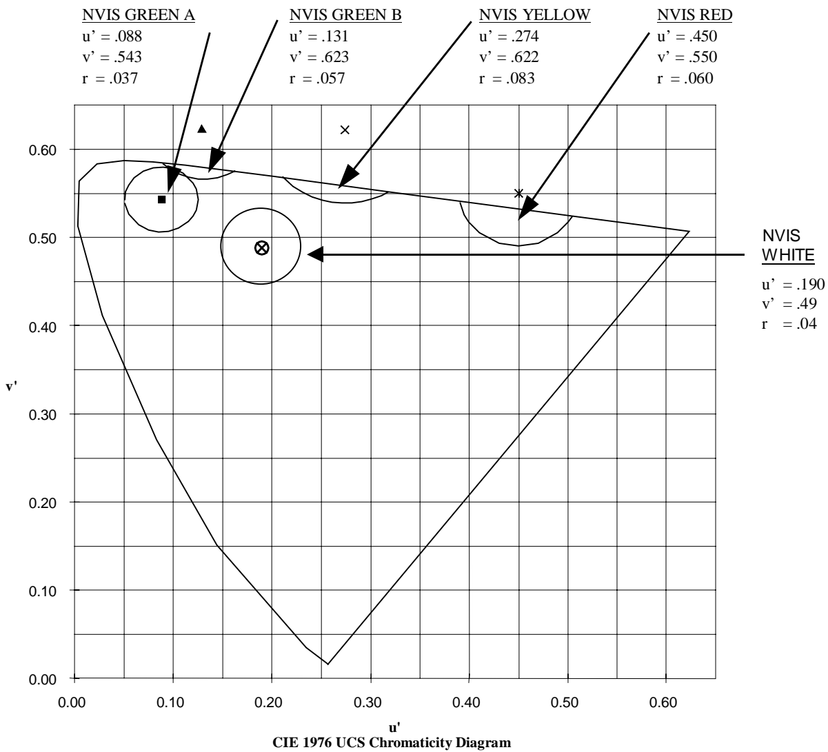
FIGURE 2. NVIS lighting color limits.
