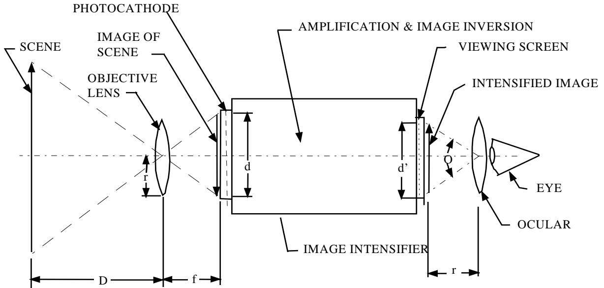
FIGURE C-1. Diagram of an image intensifier.
