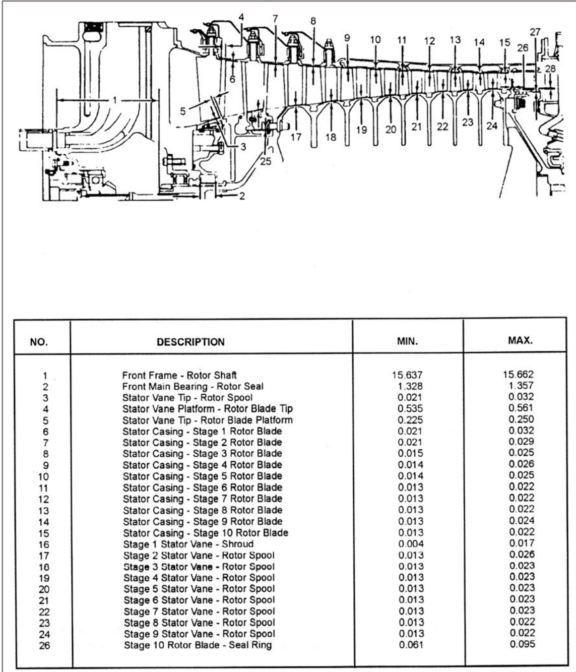
FIGURE 5. Example of dimensional data.
