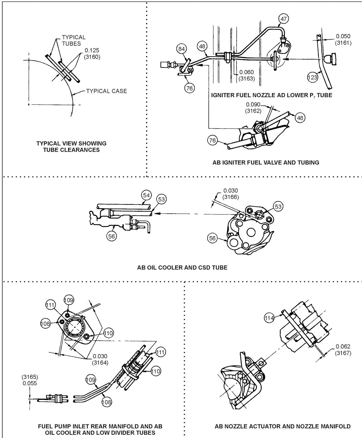
FIGURE 13. Example of critical clearances.
