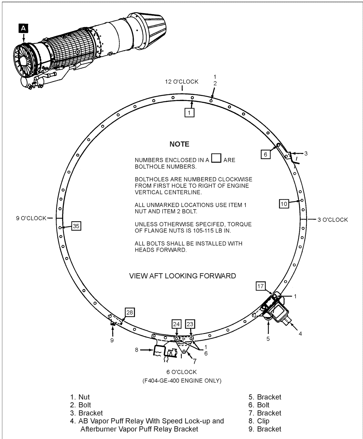
FIGURE 11. Example of a bracket installation - Continued.
