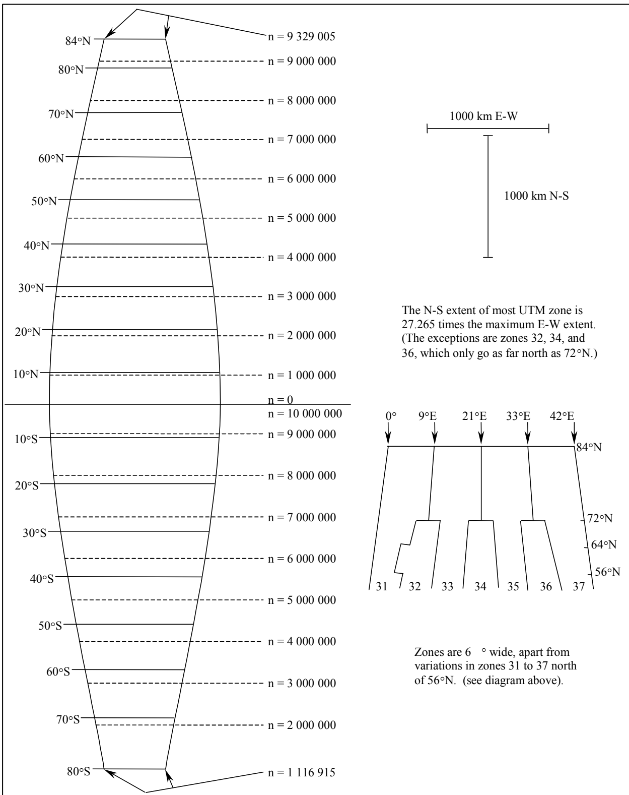
FIGURE B-1. A typical World Geodetic System 1984 (WGS 84) UTM zone (compressed).
