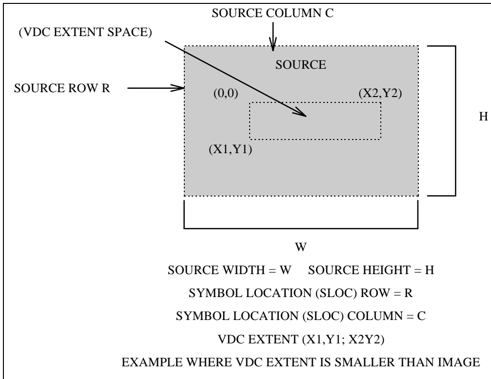
FIGURE 4. Small VDC extent output.
