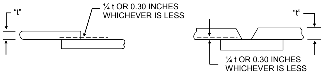
BACKING STRIP
