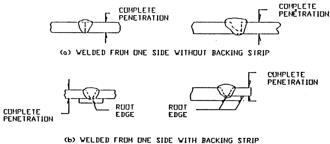
FIGURE 5-6 PENETRATION PROFILES
