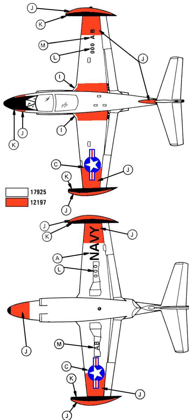
FIGURE C-22. T-2C aircraft marking (high visibility) – Continued.
