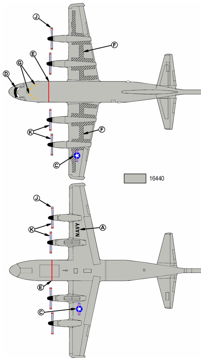
FIGURE C-19. P-3C – Continued.
