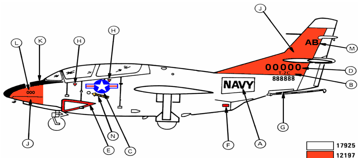
FIGURE C-22. T-2C aircraft marking (high visibility).
