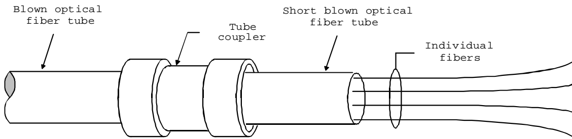
FIGURE 2F1-2. Short BOF tube and fibers.
