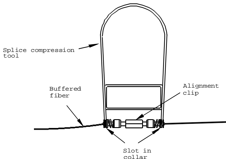
FIGURE 2C1-2. Compressing ferrule springs.
