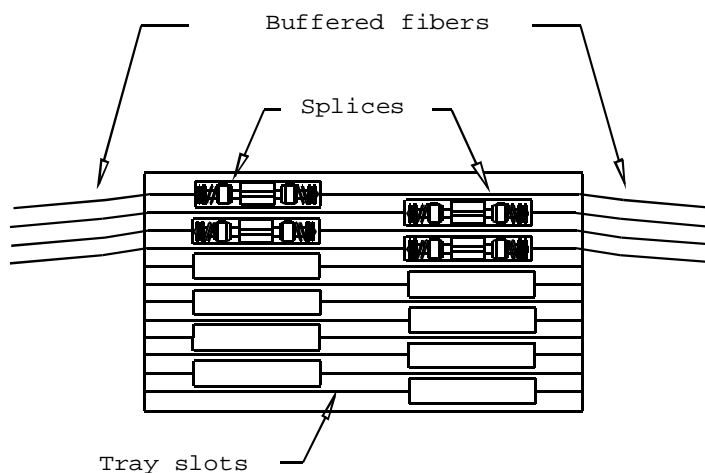
FIGURE 2C1-3. Splices installed in splice tray - (typical).
