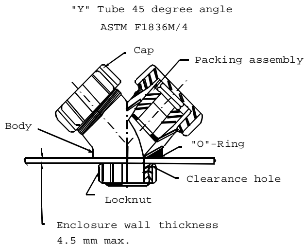
FIGURE 2G1-2. "Y" (45°) tube.
