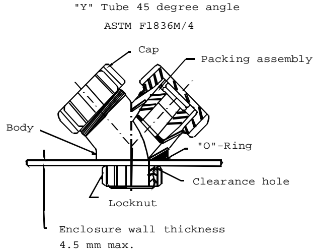
FIGURE 2A1-2. "Y" (45°) tube.
