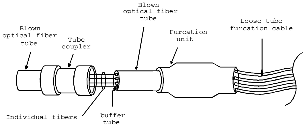
FIGURE 2F1-4. Feeding fibers into the furcation unit.
