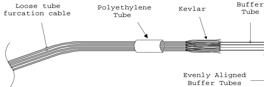
FIGURE 2E1-1. Aligning the loose tube furcation cables.
