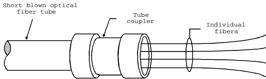
FIGURE 2F1-3. BOF tube and fibers.
