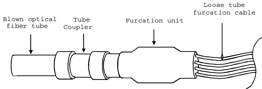
FIGURE 2F1-5. Installed furcation unit.
