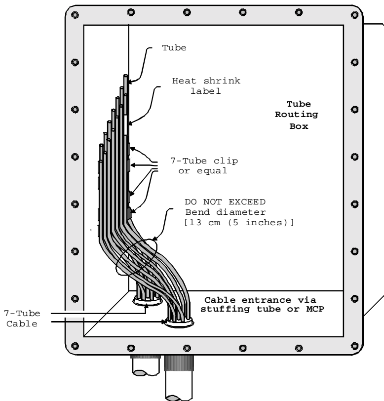
FIGURE 2I1-1. Routing BOF tubes in TRB.
