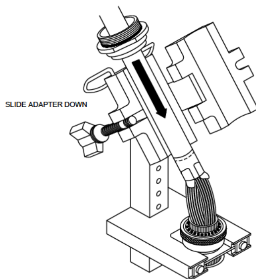
ILLUSTRATION 5 BACKSHELL ADAPTER POSITIONING
