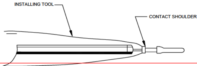
ILLUSTRATION 7 CONTACT INSERTION
