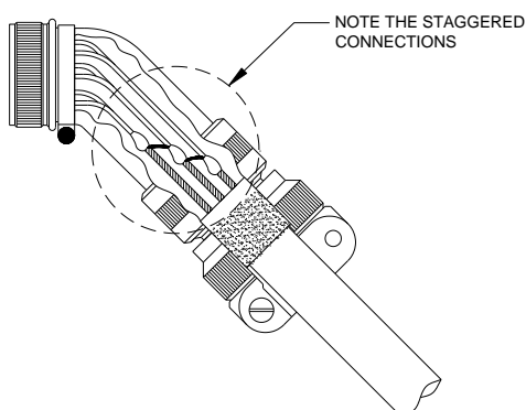
ILLUSTRATION 6 DAISY CHAIN NG SHIELD TERMINATIONS
