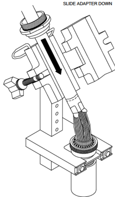
ILLUSTRATION 8 BACKSHELL ADAPTER POSITIONING
