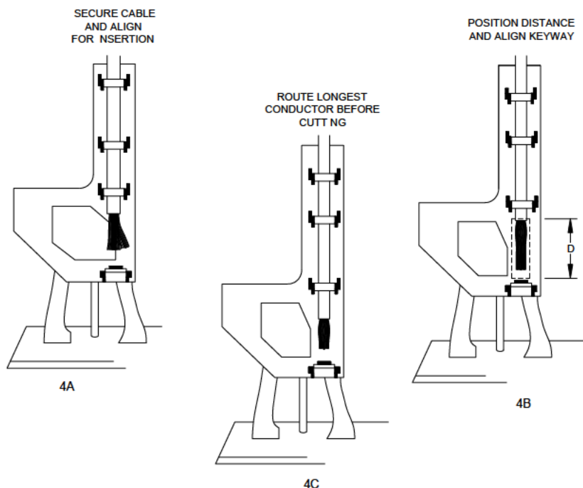
ILLUSTRATION 4 DETERMINING CONDUCTOR LENGTH
