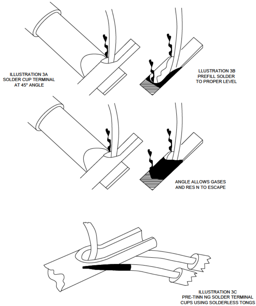
ILLUSTRATION 3 - PRE-TINNING THE SOLDER TERMINAL CUPS
