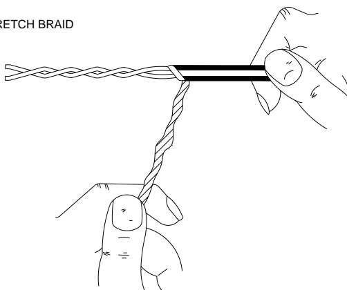
ILLUSTRATION 8 INDIVIDUAL SH ELD TERMINATION
