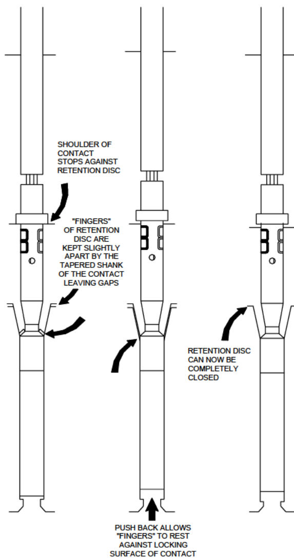
ILLUSTRATION 7 CONTACT "PUSH-BACK"
