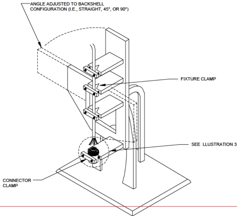
ILLUSTRATION 2 ASSEMBLY FIXTURE
