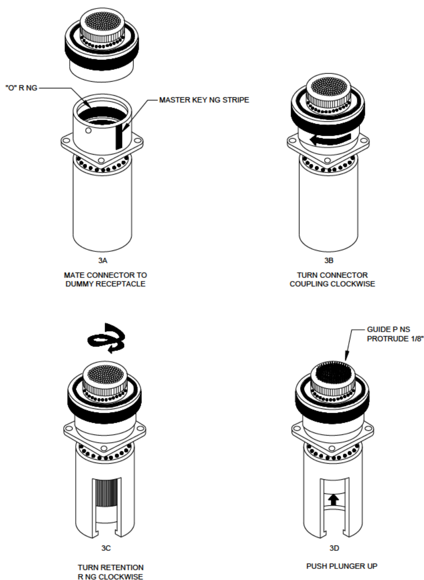
ILLUSTRATION 3 DUMMY RECEPTACLE
