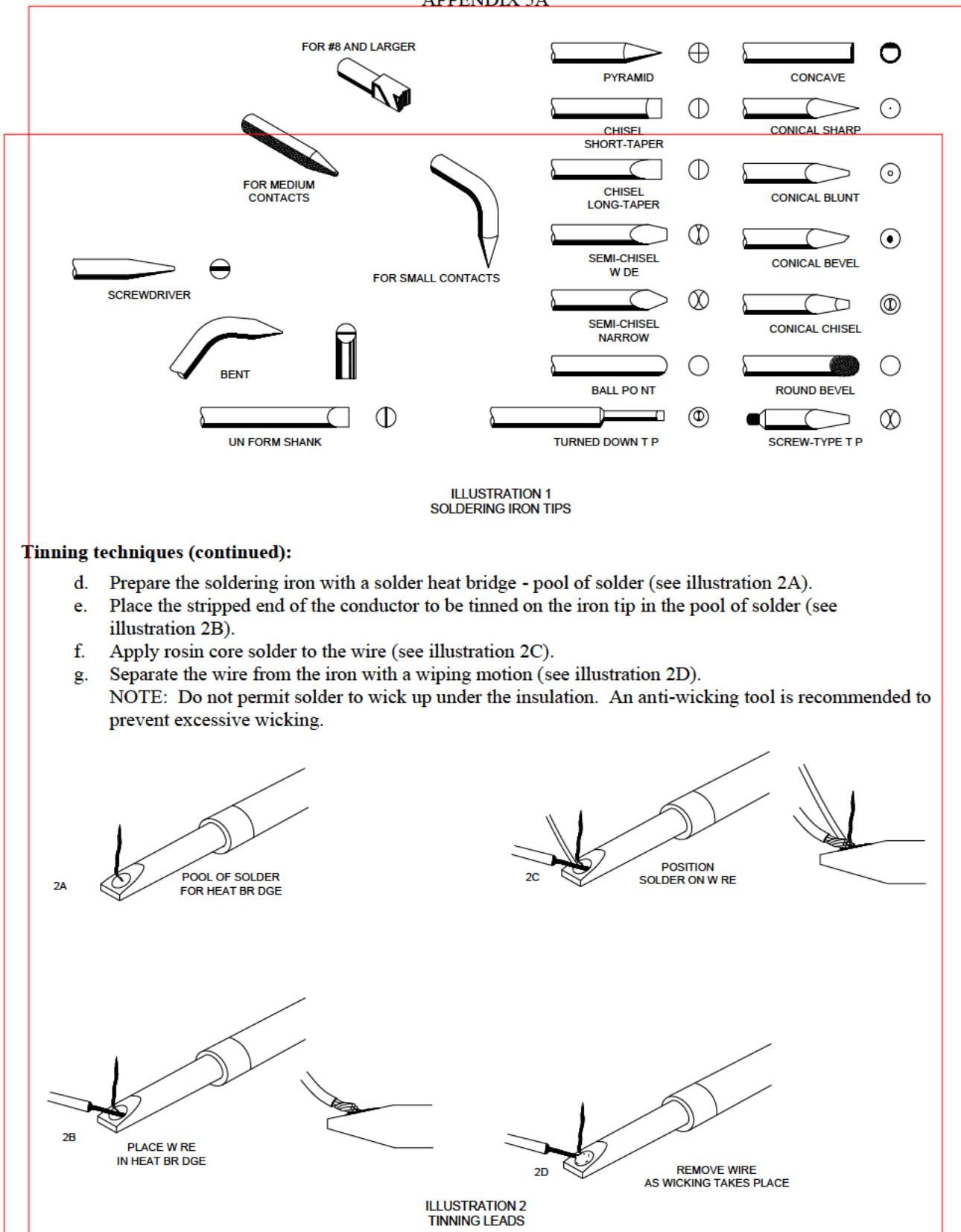
FIGURE 5A5. Tinning techniques – Continued.
