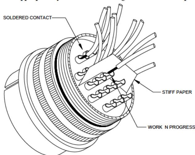
ILLUSTRATION 5 PROTECT NG SOLDERED CONTACTS
