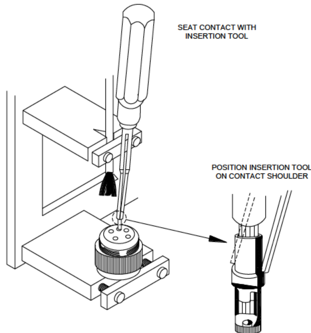
ILLUSTRATION 6 CONTACT INSERTION
