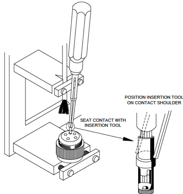
ILLUSTRATION 5 CONTACT INSERTION
