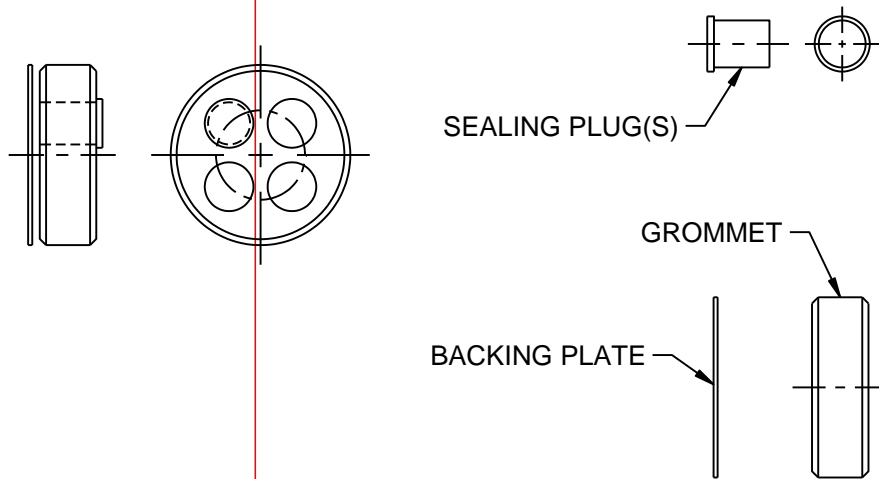
Illustration 14, Typical Glenair grommet plugs, grommet (side view), and backing plate
