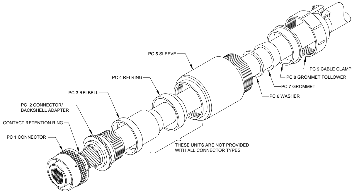
ILLUSTRATION 1 SAE-AS81511 CONNECTOR WITH COMPATIBLE BACKSHELL CONFIGURATION
