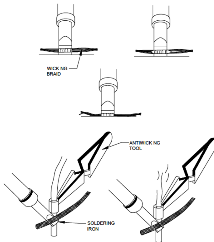
ILLUSTRATION 7 - BRAIDED WICK WIRE SOLDER REMOVAL
