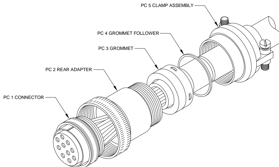
ILLUSTRATION 5 TYPICAL SAE-AS50151 (MOD F ED) CONNECTOR/BACKSHELL CONFIGURATION
