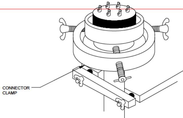
ILLUSTRATION 3 CONNECTOR SEATED IN ASSEMBLY FIXTURE
