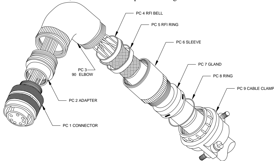
ILLUSTRATION 1 MIL-DTL-27599 CONNECTOR WITH COMPATIBLE BACKSHELL CONFIGURATION
