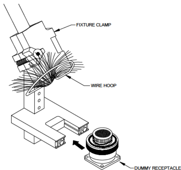
ILLUSTRATION 2 ASSEMBLY FIXTURE
