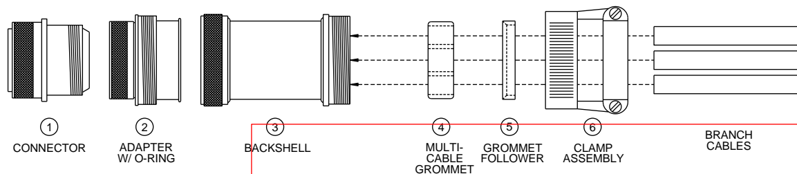
Illustration 1, Multi-Cable Connector Assembly
