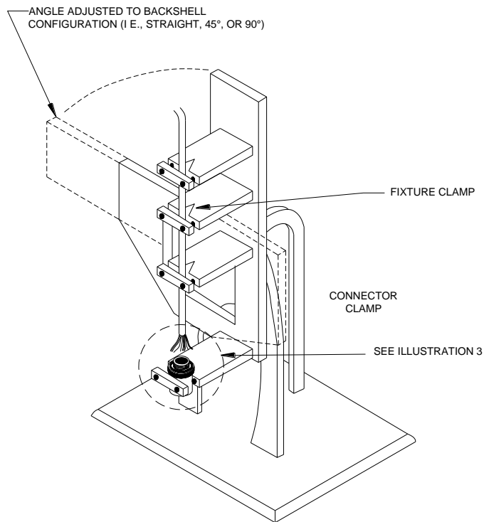
ILLUSTRATION 2 ASSEMBLY FIXTURE
