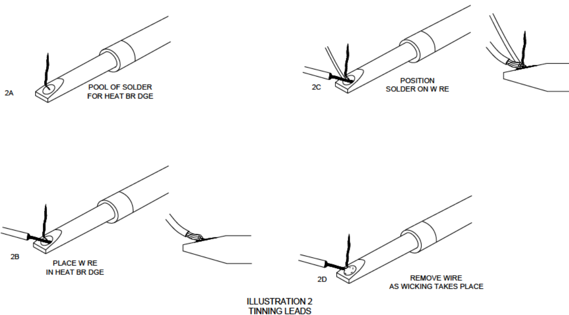
FIGURE 5A5. Tinning techniques – Continued.
