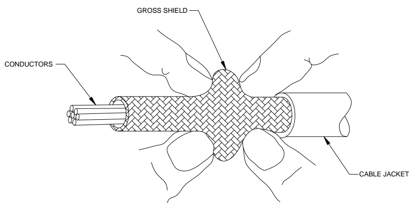
ILLUSTRATION 2 GROSS SHIELD INTERFERENCE REMOVAL
