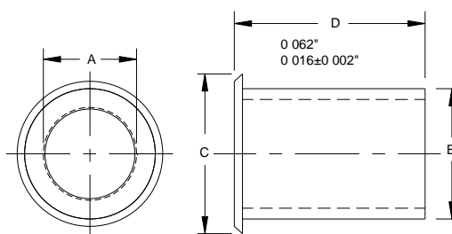
ILLUSTRATION 3 SAE-AS85049
