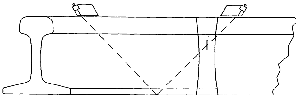
6-A Dual search unit positioning for through-transmission evaluation of discontinuities detected using the shear wave inspection technique while scanning from the running surface.
