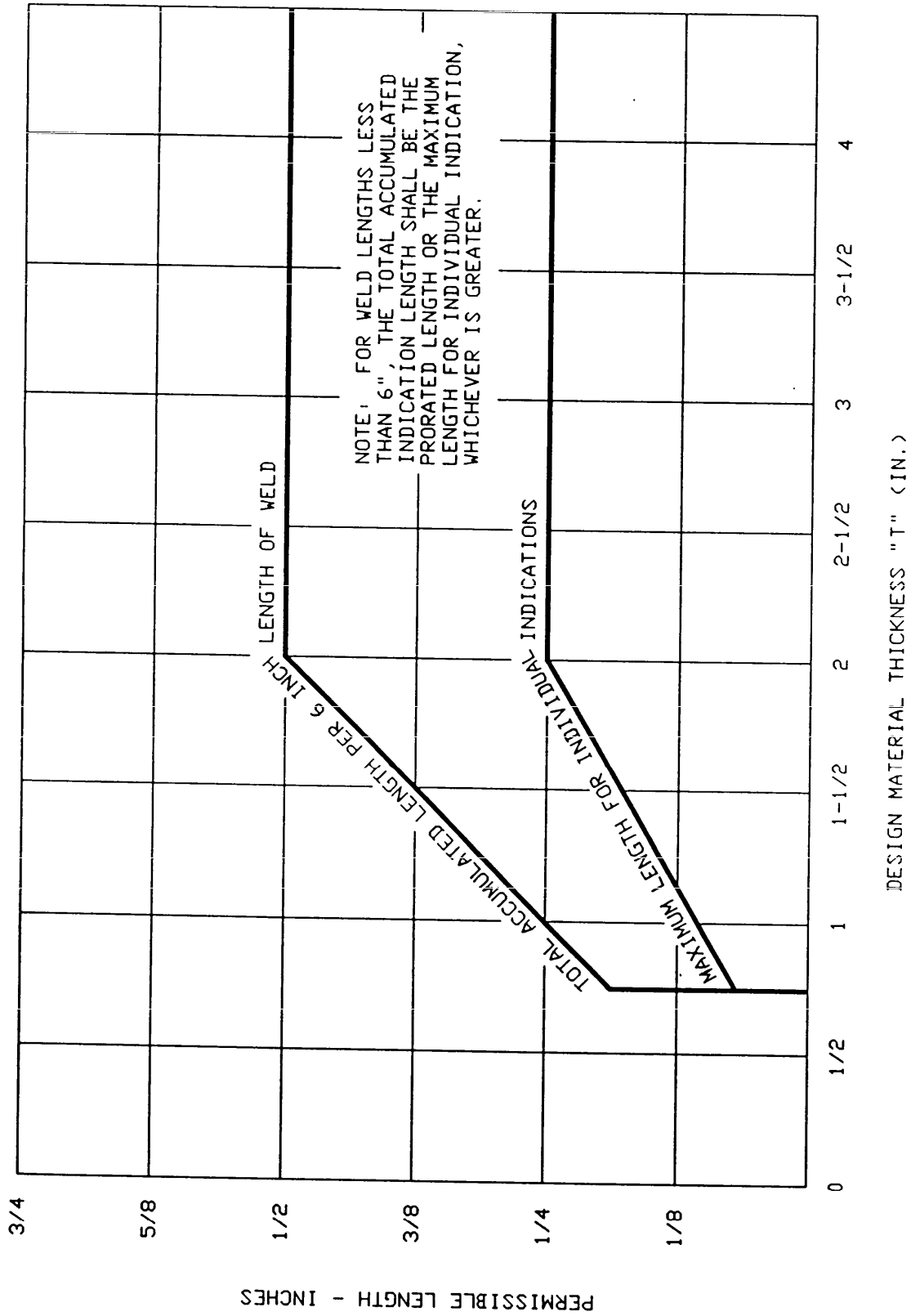
FIGURE 8. Production weld, acceptance standard for incomplete fusion and incomplete penetration indications.
