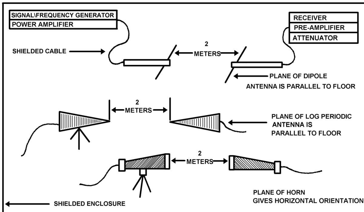
FIGURE 3308-1. Dynamic range and isolation measurements.
