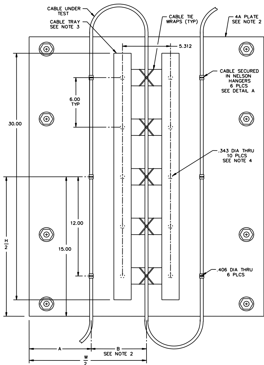
FIGURE 3202-4: Supplemental test fixture for cable of small diameter.
