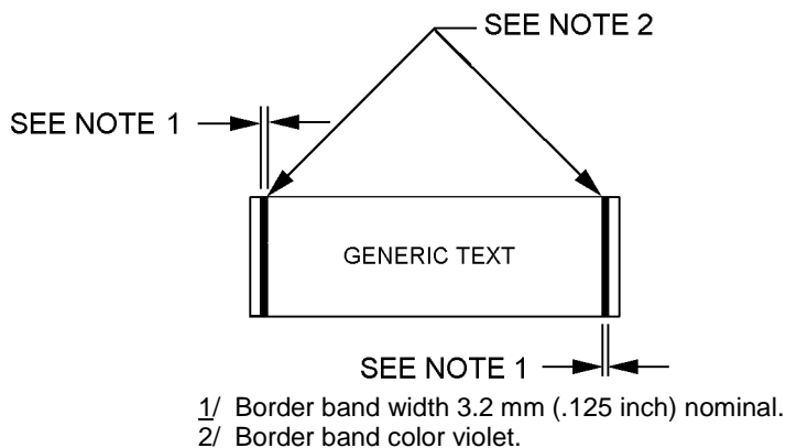
FIGURE 1104 B-1. One cable harness marking scheme.
