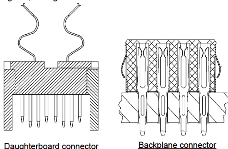
FIGURE A-4. Section view of daughterboard and backplane connectors.
