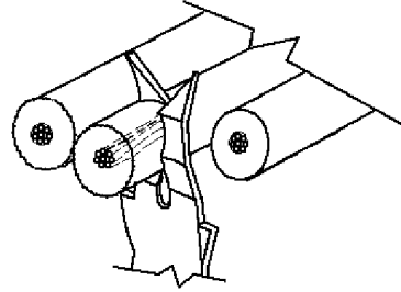
FIGURE A-2. Insulation displacement contact (IDC).
