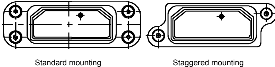
FIGURE B-1. MIL-DTL-83733, mounting configurations.
