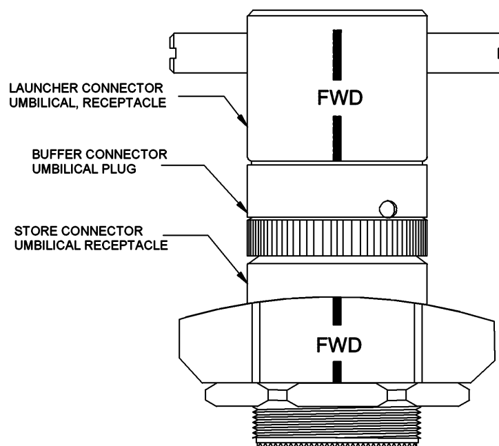
FIGURE D-1. Electrical umbilical assembly .
