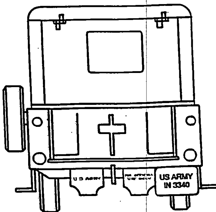
FIGURE 18. Utility truck with Army markings.
