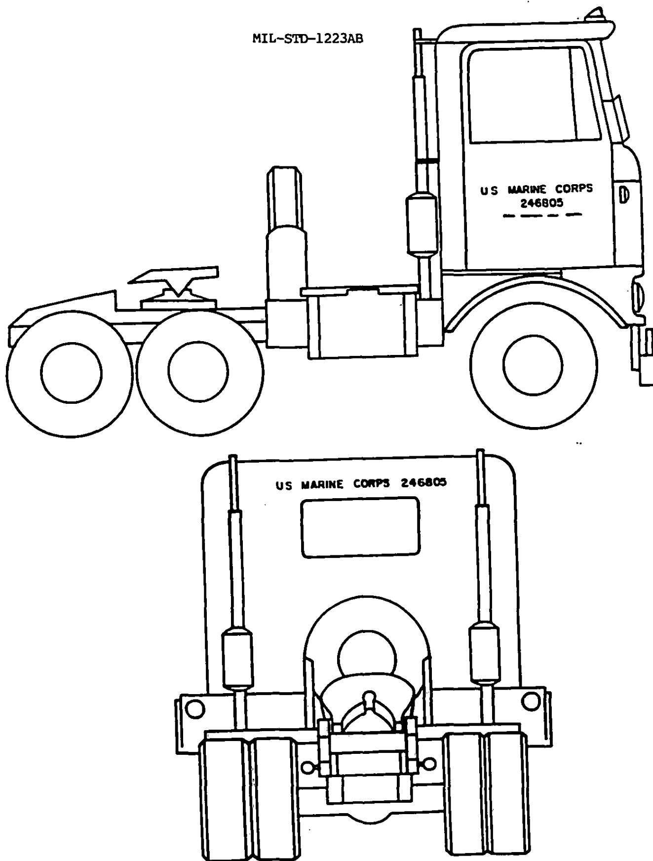
FIGURE 15. Truck Tractor with Marine Corps markings.
