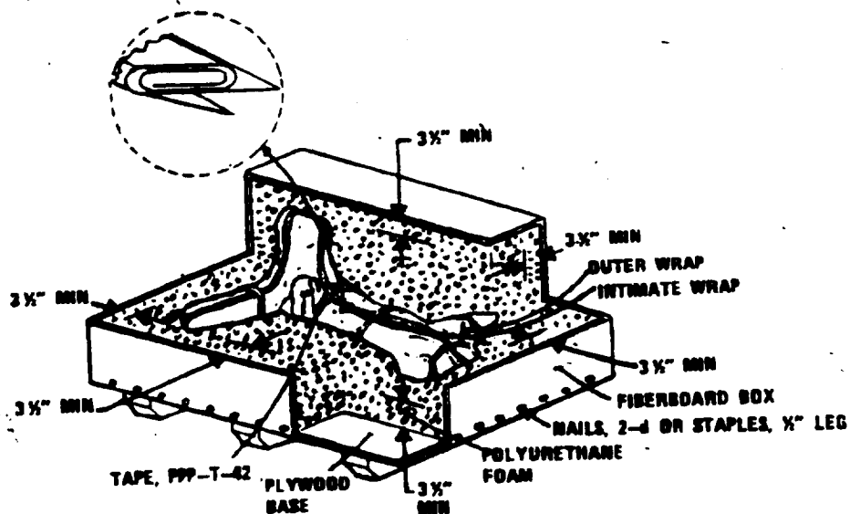
FIGURE 11. Encapsulated pack (design 3).
