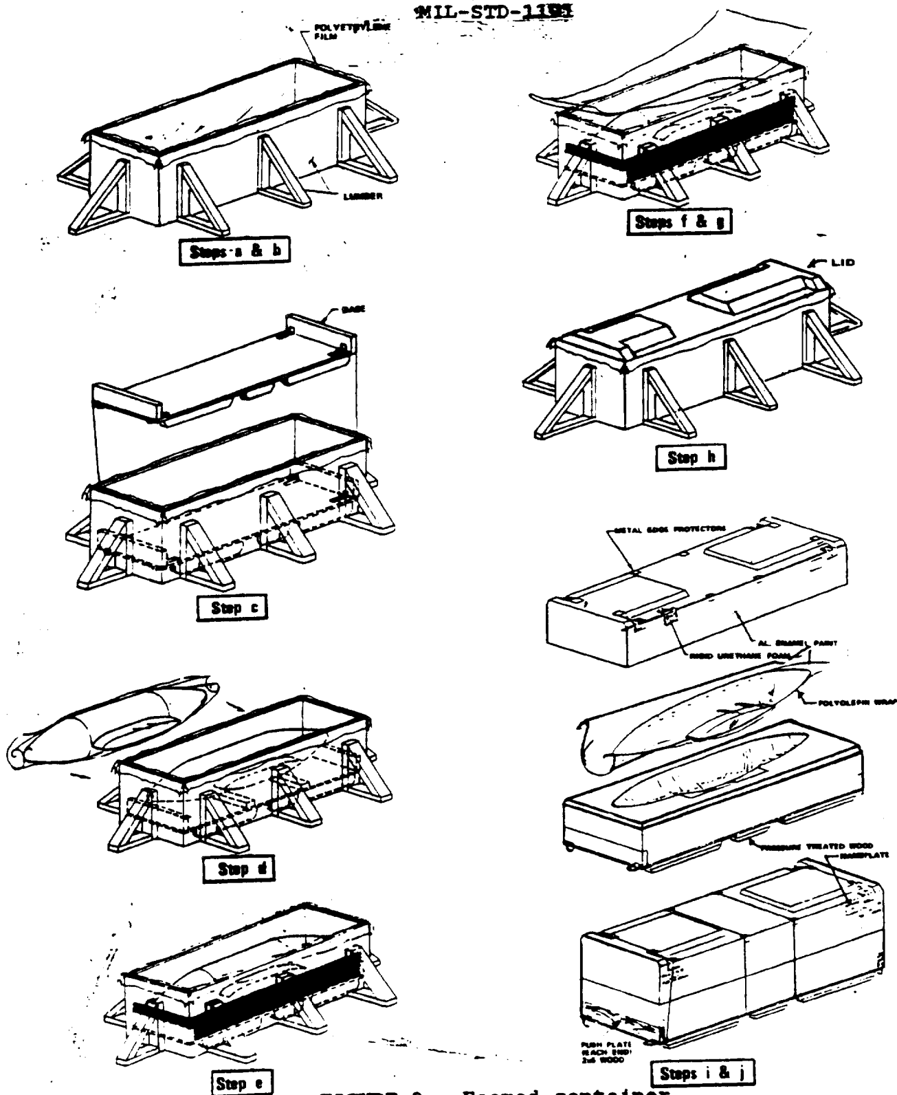
FIGURE 8. Foamed container.
