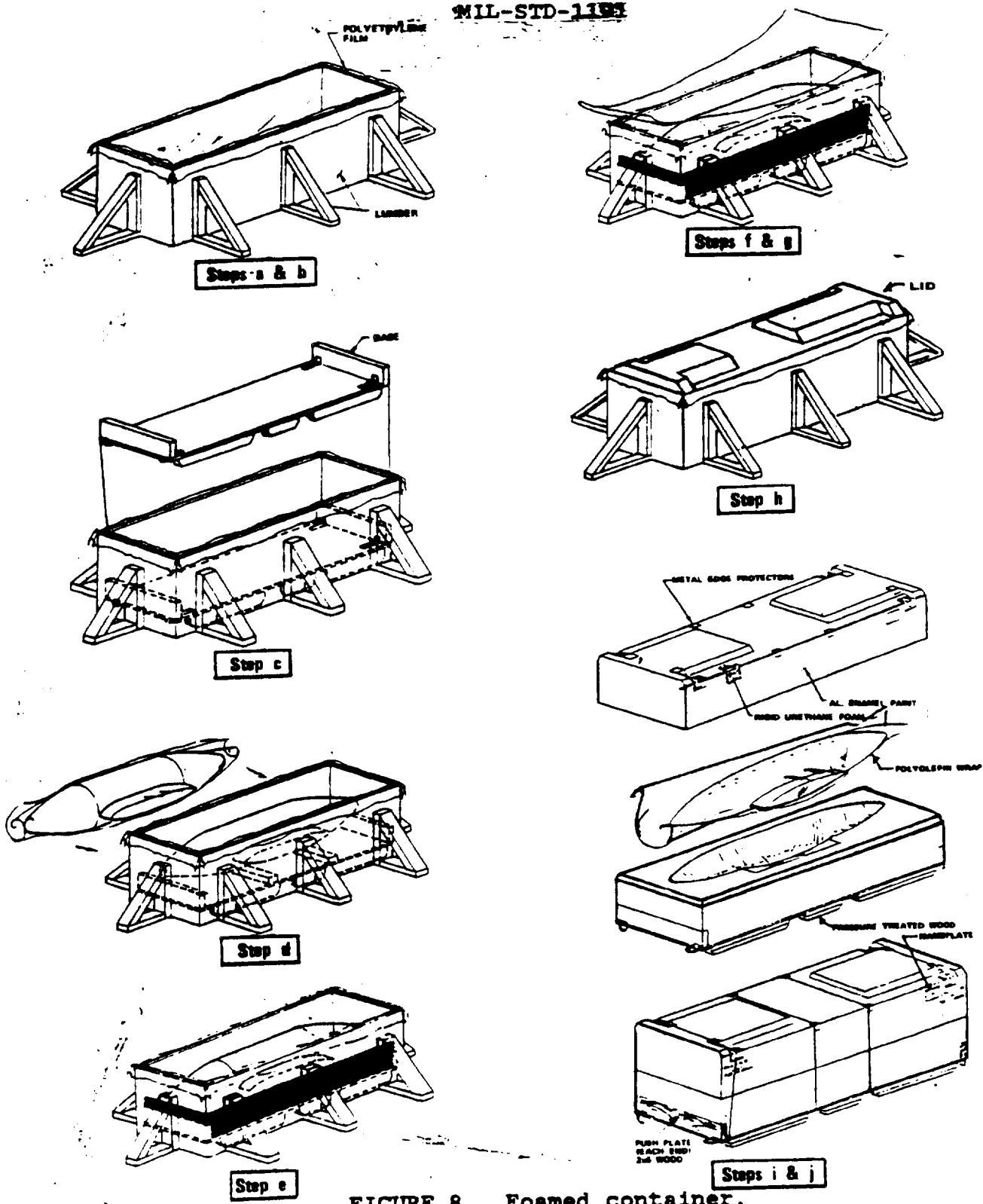
FIGURE 8. Foamed container.
