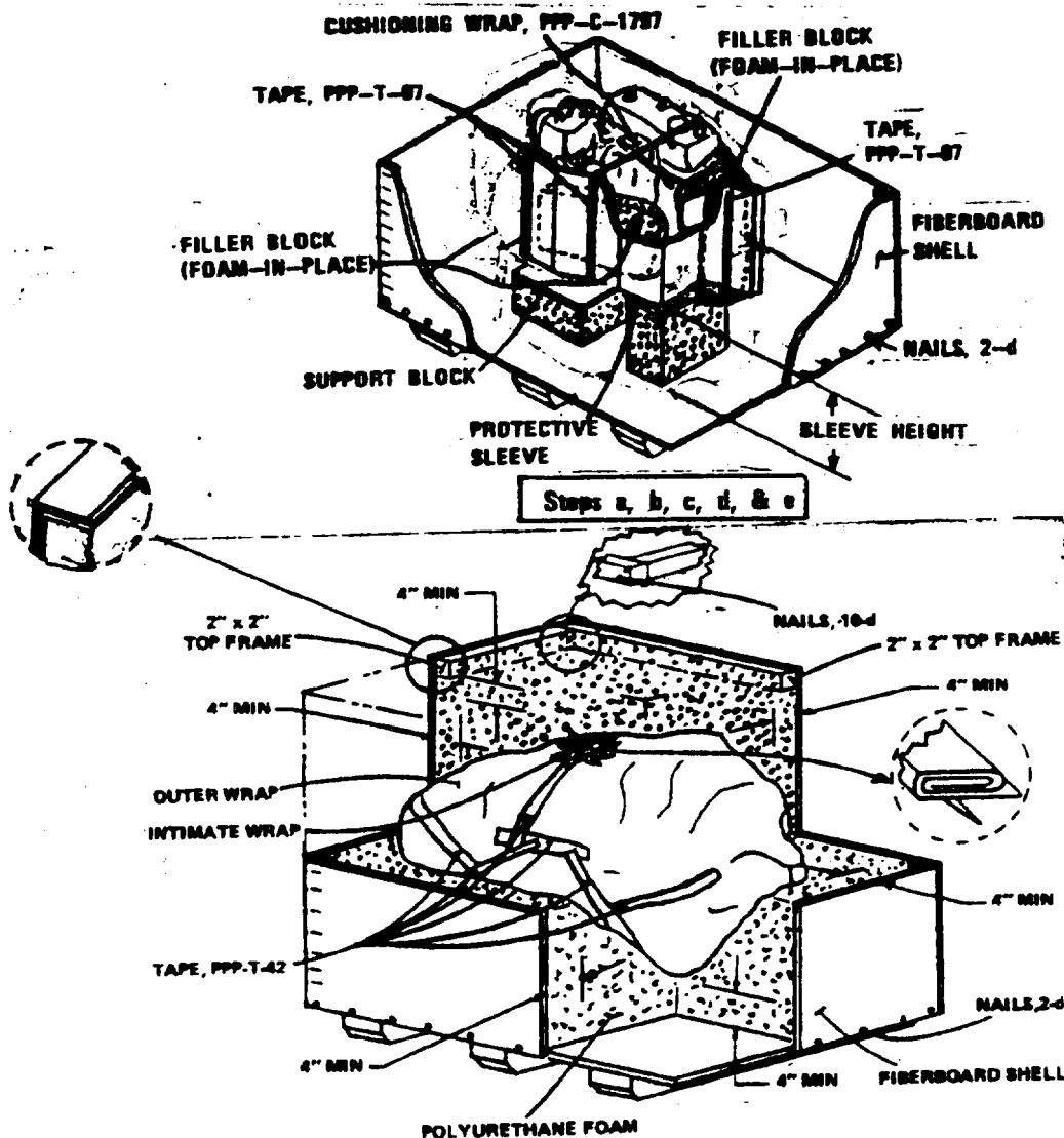
FIGURE 12. Encapsulated pack (design 4).
