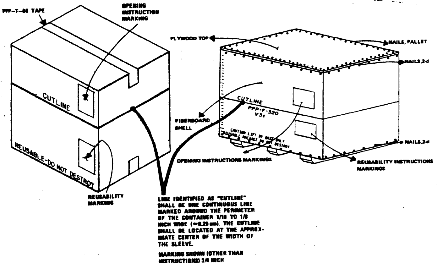
FIGURE 13. Encapsulated pack, special marking locations.
