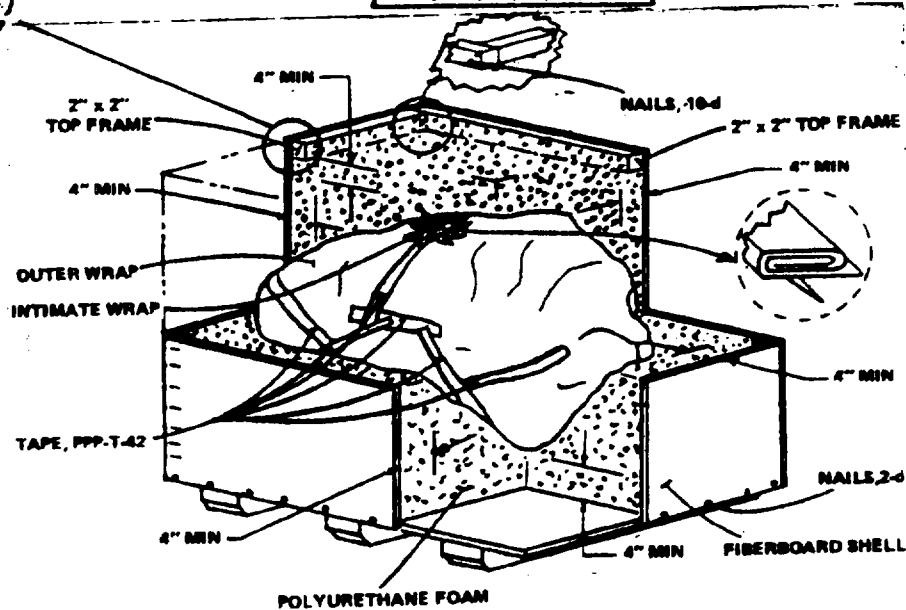
FIGURE 12. Encapsulated pack (design 4).
