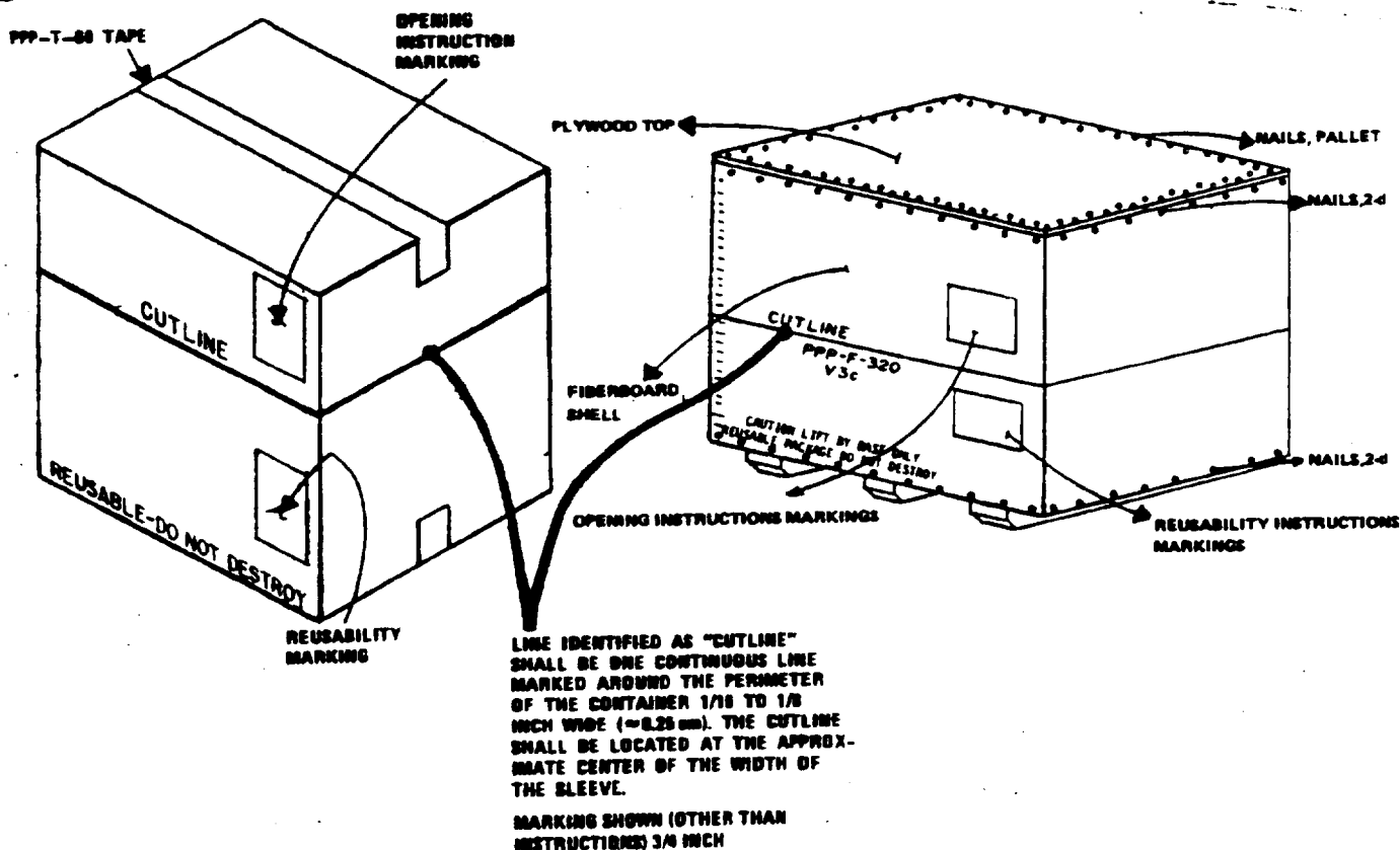
FIGURE 13. Encapsulated pack, special marking locations.
