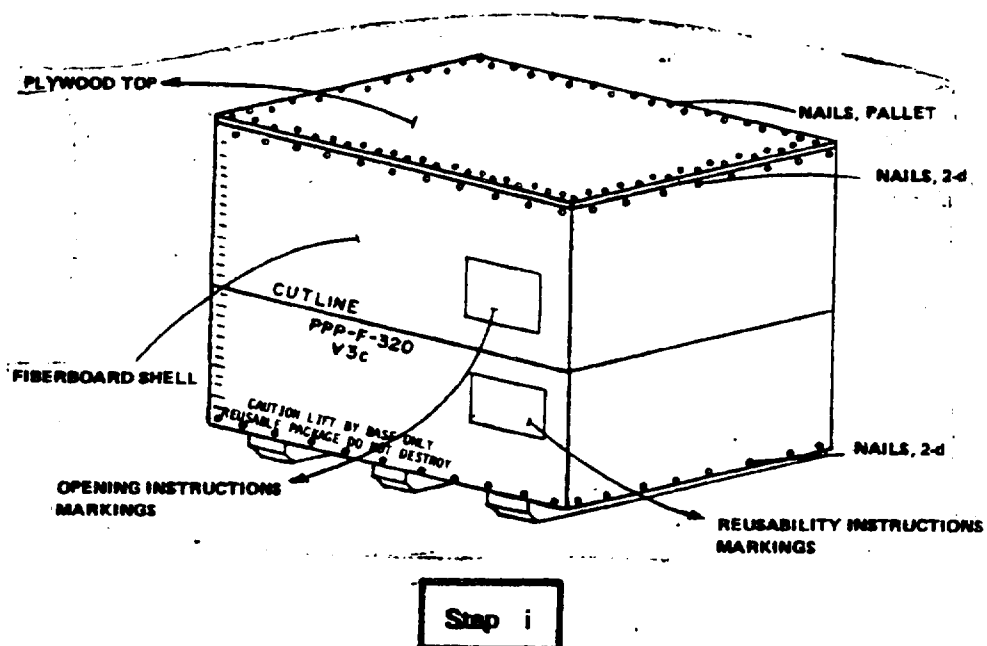
FIGURE 12 Encapsulated Pack (design 4) --Continued.
