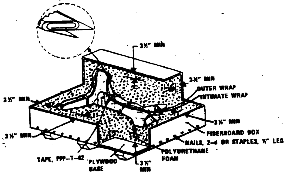
FIGURE 11. Encapsulated pack (design 3).
