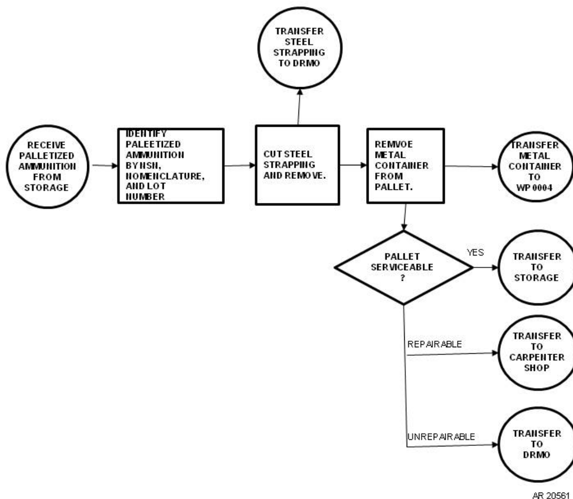
Figure 1. Flowchart for Unload Pallet (Skid).
