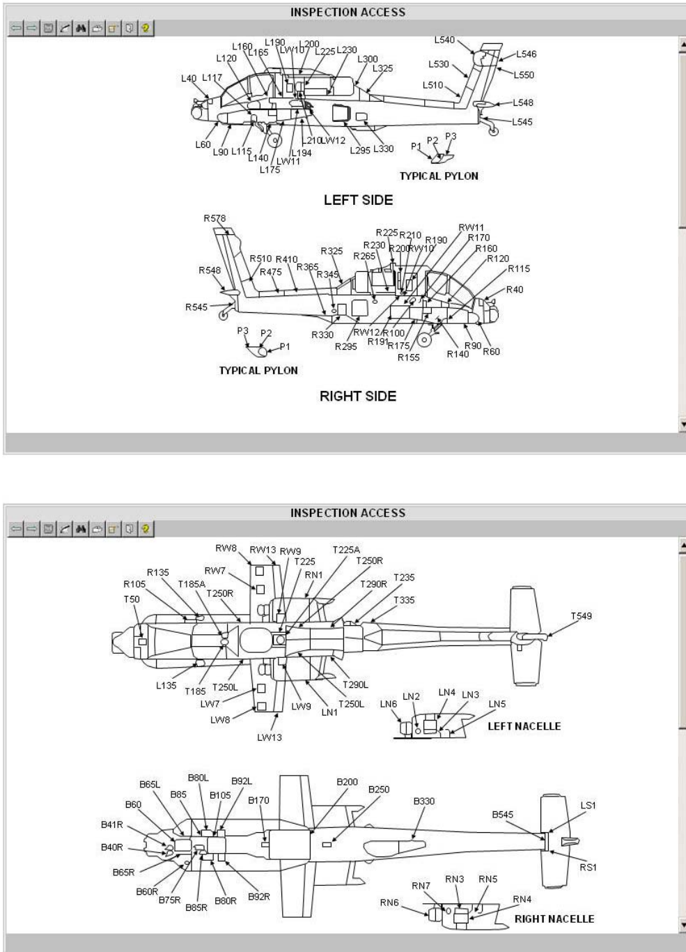
FIGURE E-11. Example of inspection access provisions.
