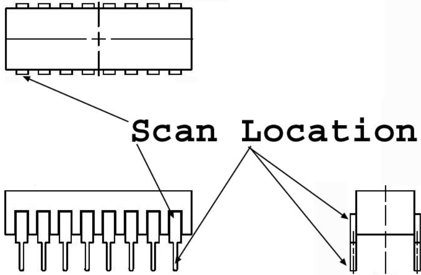
FIGURE 2037-5. Scan Locations on Dual In-Line Package.
