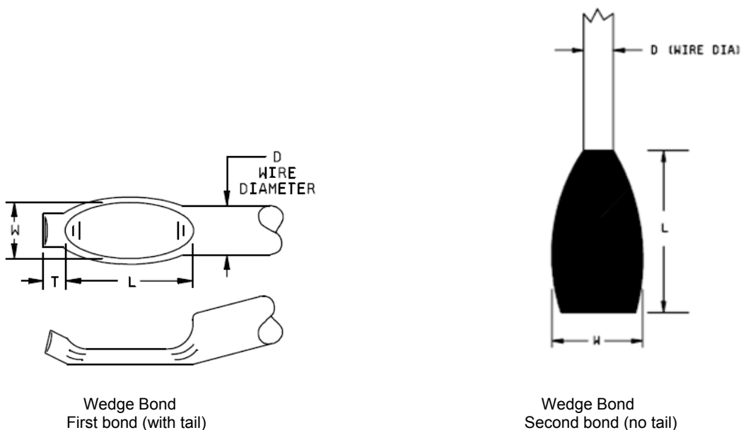
Figure 2017-16a. Bond Dimensions .
