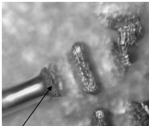
Reject bond is cracked at the heel. Figure 2017-20e.
