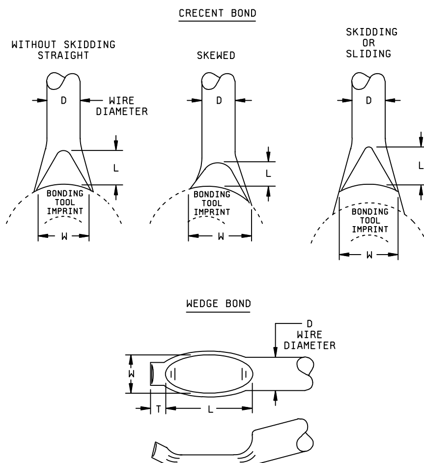
FIGURE 2010-33. Bond dimensions .
