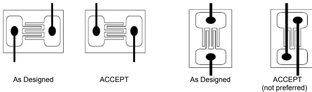
Figure 2017-14. Acceptable Symmetrical Element Orientation.
