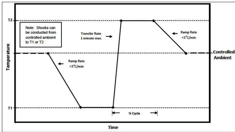
Figure 503.6-1. Single Shocks (1/2 cycle).
