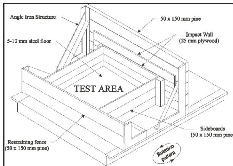
Figure 514.7C-5. Category 5 - Loose cargo test setup.
