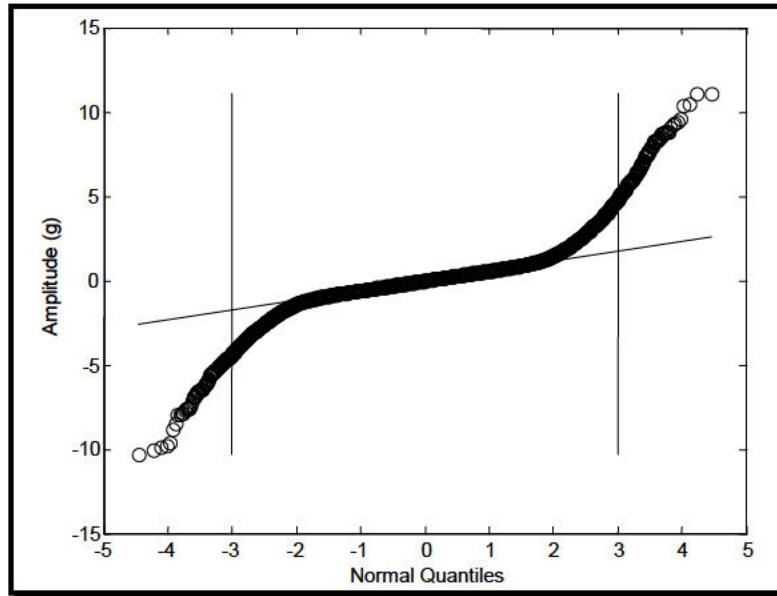
Figure 519.7B-11a. qq-plot, gunfire shock time trace difference (2000 rnd/min).
