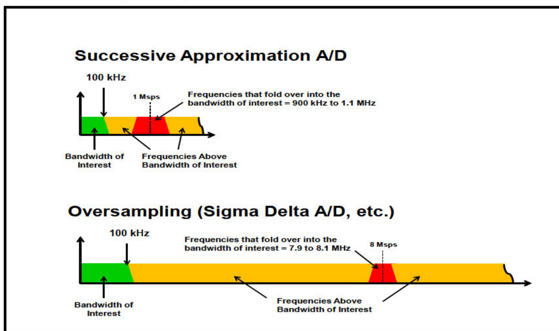
Figure 517.2-8. Illustration of sampling rates and out of band “fold over” frequencies for data acquisition systems.
