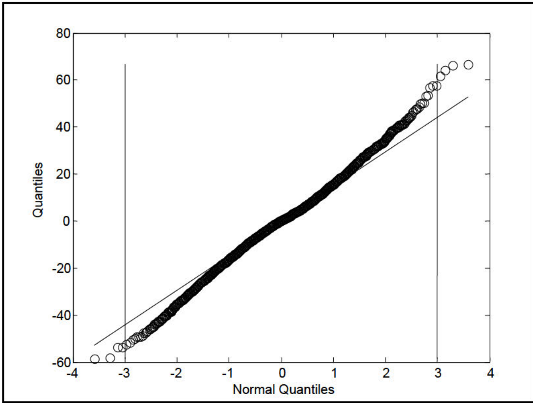
Figure 519.7B-7b. qq-Plot for composite random component decomposition 4000 rnd/min.
