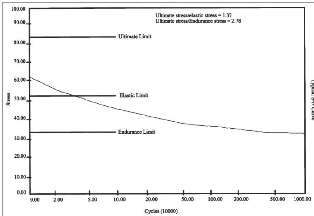
Figure 515.7F-6. Typical S-N curve.
