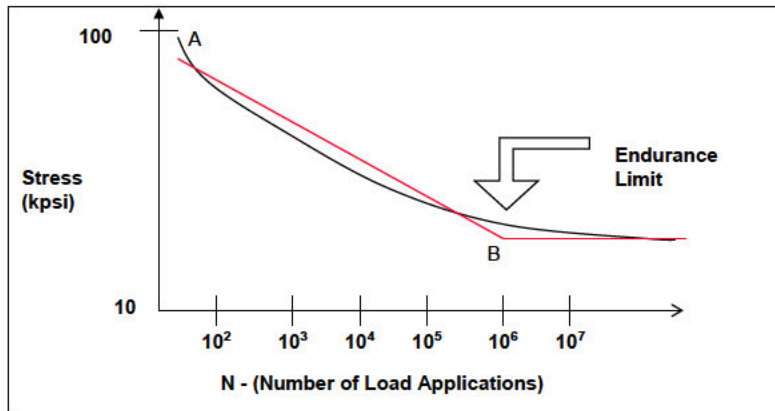
Figure 514.7F-2. S/N curve.
