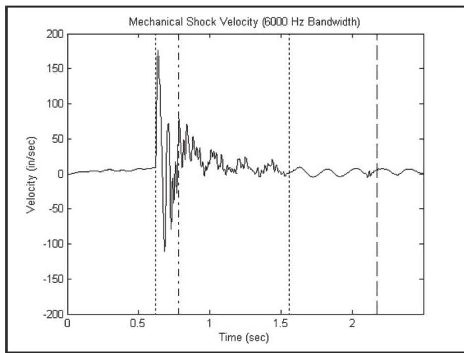
Figure 516.7A-4. Measurement velocity via integration of mean (DC) removed acceleration.
