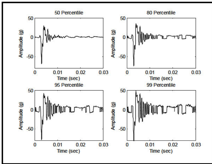
Figure 519.7E-2. Ensemble quantile (percentage point) plot.
