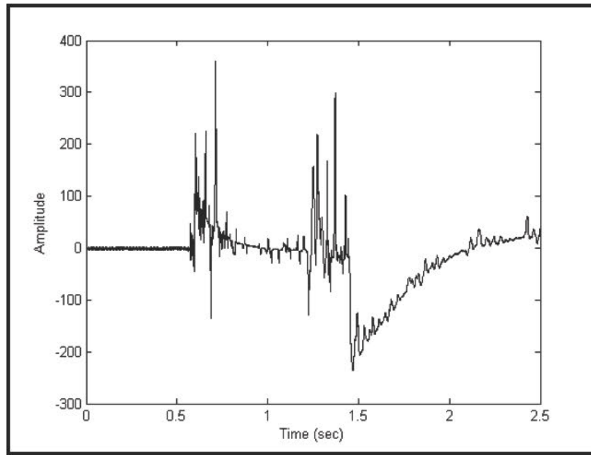
Figure 516.7A-9. Combination amplifier overdriving and noise.
