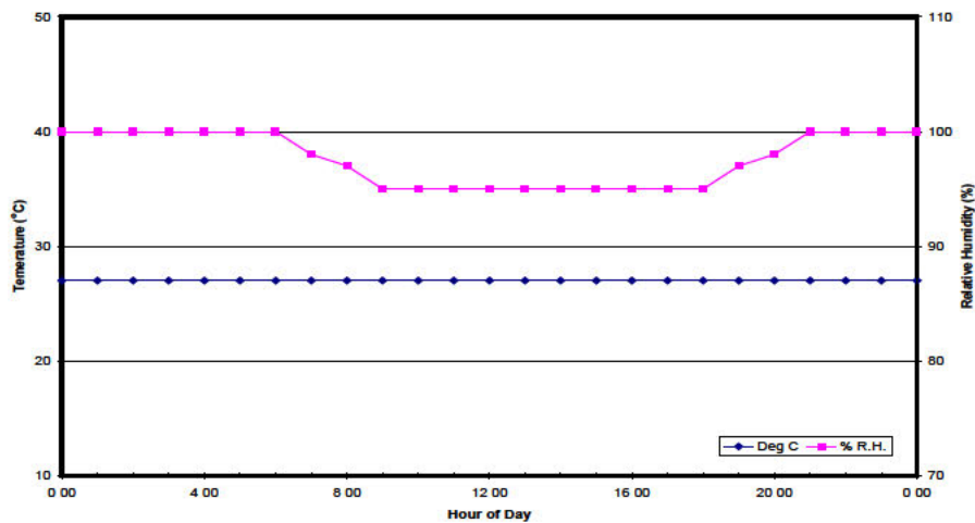
Figure 507.6-1. Induced Cycle B1 - Storage and transit.
