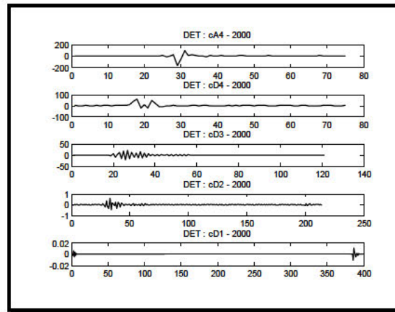
Figure 519.7B-6a. Wavelet decomposition for deterministic component, (db15) (2000 rnd/min).
