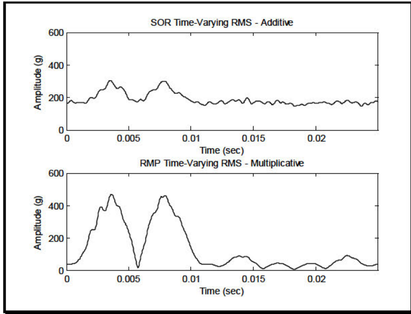
Figure 519.7C-9c. Pulse ensemble statistics - root-mean-square \sqrt{(m(t)+r(t))^2} .
