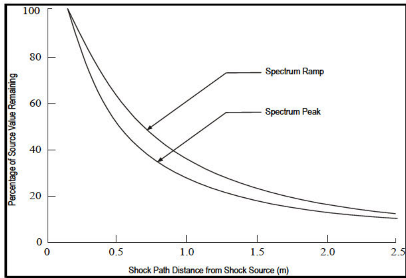
Figure 517.2-11. Shock response spectrum versus distance from pyrotechnic source.
