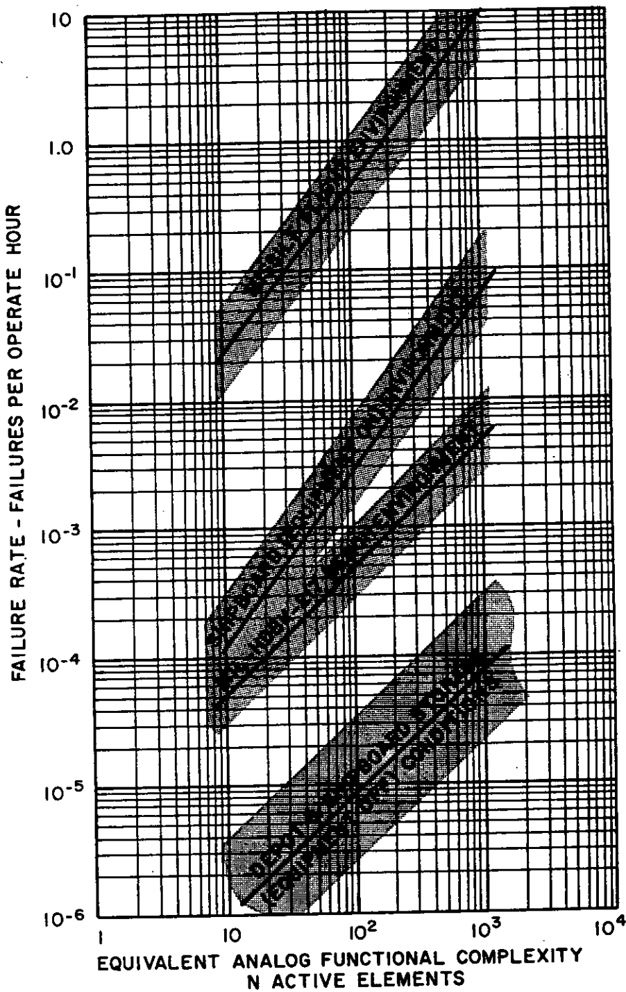
Figure 2003.1. Failure-Rate Estimating Chart for Electronic Analog Function.
