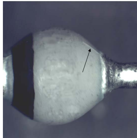
FIGURE 2068-1. Critical glass and meniscus areas for nontransparent glass, double plug, noncavity diodes.
