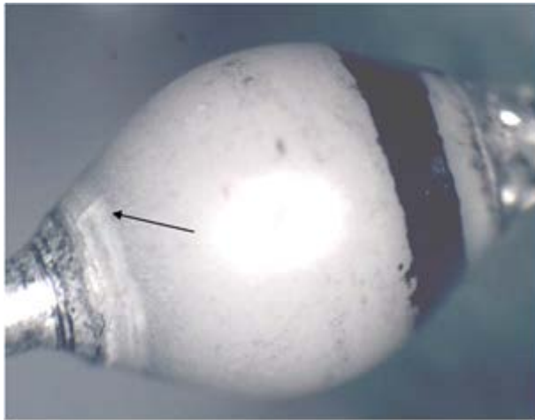
FIGURE 2068-1. Critical glass and meniscus areas for nontransparent glass, double plug, noncavity diodes.
