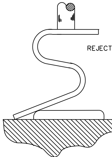
FIGURE 2074-A6. Whisker toe contact on top surface of die.
