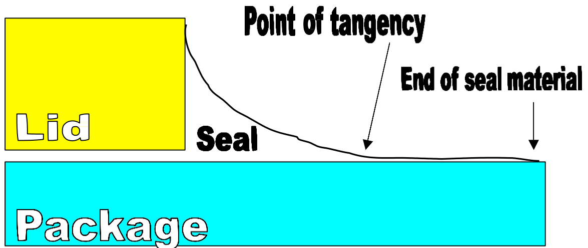
FIGURE 2076-7. Design sealing width and seal fillet graphic.
