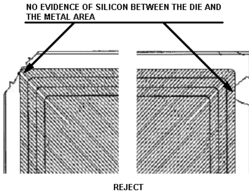
FIGURE 2078-5. Cracks and chips (continued).
