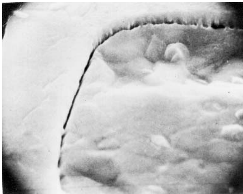
FIGURE 2077-11. Separation of metallization at contact step at 7,000X (reject).
