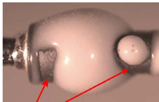
FIGURE 2068-5. Unacceptable body glass coverage.
