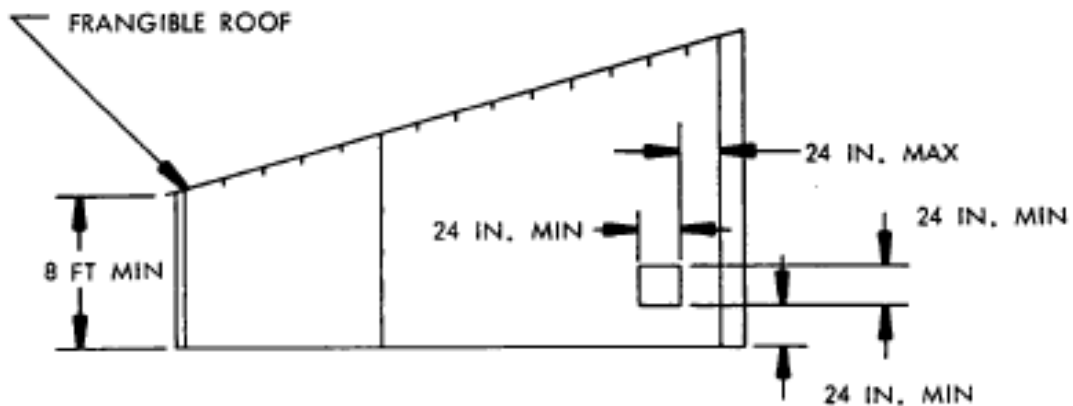
FIGURE 1. Simulated operational bay environment .
