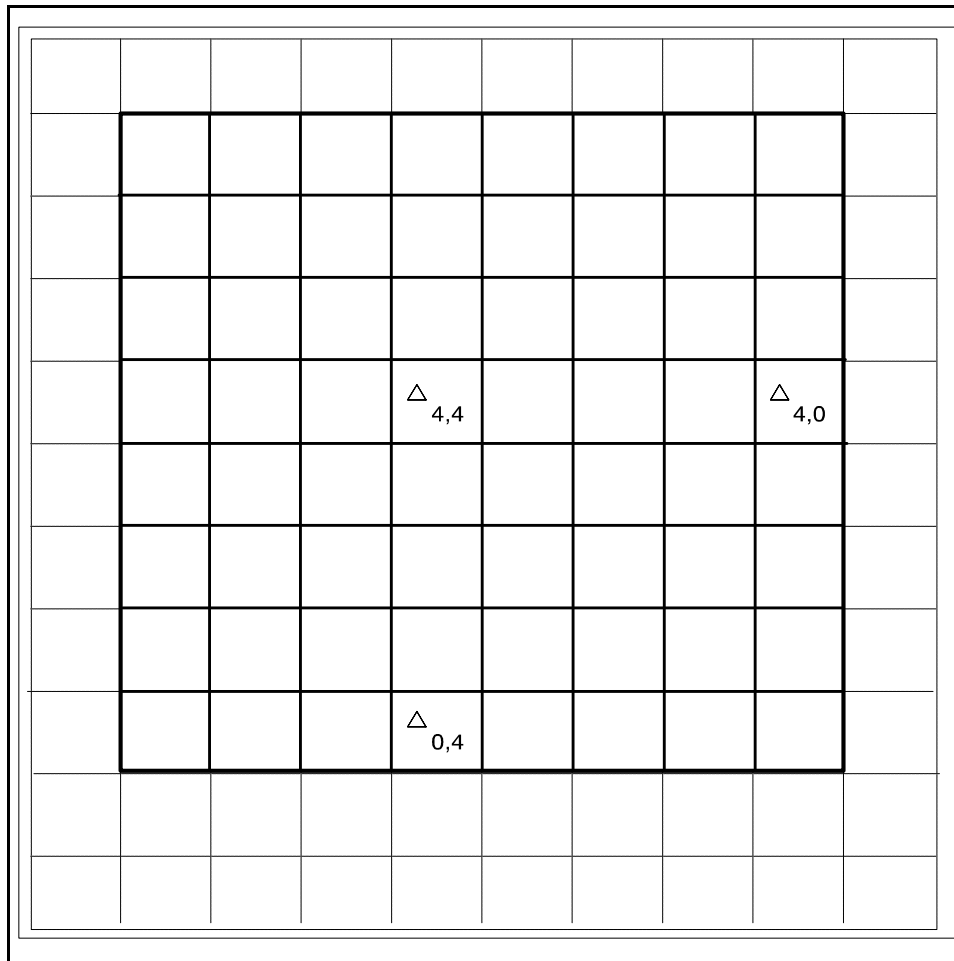
FIGURE 5. Level 2 deltas.
